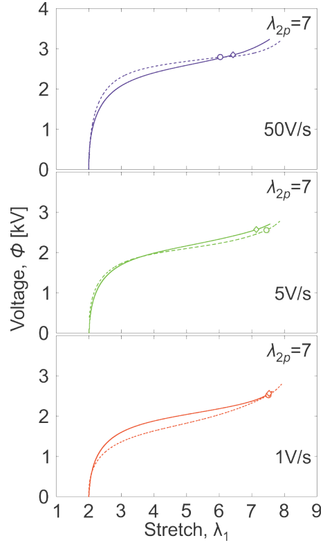
Fig. 5 Voltage-stretch curves for the membrane of prestretches \{2, 7\} at voltage ramp rates of 1V/s, 5V/s and 50 V/s. The solid curves represent the experimental data, while the dashed curves represent the theoretical calculations. The circles and diamonds represent the points at which the membrane suffers loss of tension in the theoretical predictions and experimentally observations, respectively. The material parameters used in the calculations are \mu^\alpha = 20\text{kPa} , \mu^\beta = 200\text{kPa} , J_{\text{lim}}^\alpha = 155 , J_{\text{lim}}^\beta = 155 , \eta / \mu^\beta = 50 , and \varepsilon = 4.12 \times 10^{-11} \text{F/m} .
