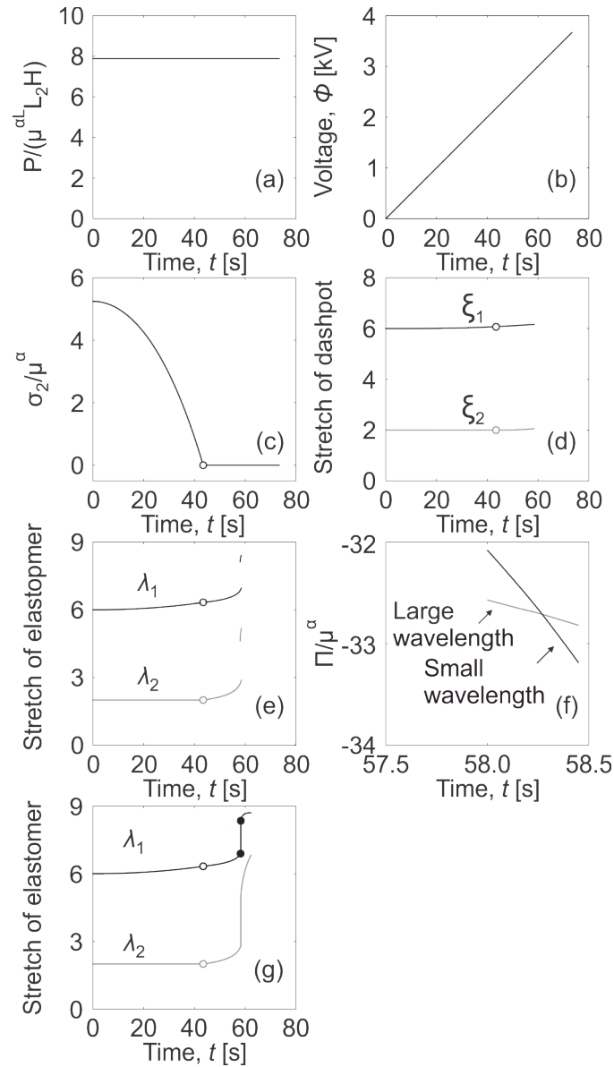
Fig. 9 Evolution and snap in the membrane of pre-stretches \{6, 2\} at a voltage ramp rate of 50 V/s. (a) The membrane is subject to a constant load in the vertical direction. (b) Voltage increases at a ramp rate of 50 V/s. (c) Horizontal tensile stress reduces as the voltage increases. At t = 43.4 s, the horizontal tensile stress vanishes. The loss of tension is indicated as open circles and causes the membrane to form wrinkles. (d) Evolution of the dashpot deformation. (e) Evolution of the elastomer deformation. When t = 58 s, another wrinkled state of equilibrium exists with a small wavelength. (f) Energy densities of the two wrinkled states. One has a small wavelength; the other has a large wavelength. When t = 58.3 s, the two wrinkled states have the
