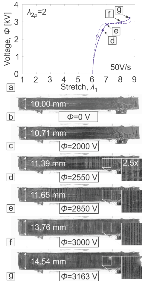
Fig. 10 (a) Voltage-stretch curves for the membrane of prestretches \{6, 2\} at a voltage ramp rate of 50 V/s. The solid curve represents the experimental data, while the dashed curve represents the theoretical predictions. The open circle indicates the calculated loss of tension while the diamond notifies the experimental observation respectively. The membrane exhibits a continuous transition from the flat state to the wrinkled state, and then exhibits a discontinuous transition from the wrinkled state with a large wavelength to that with a small wavelength. (b-g) Experimental observations. (b) The membrane is flat, subject to no voltage. (c) The membrane is still flat, when the voltage is small. (d) The membrane suffers loss of tension, and exhibits a continuous transition from the flat state to the wrinkled state at \Phi = 2550\text{V} . (e-f) The membrane suffers snap through instability at \Phi = 2850\text{V} , and exhibits a discontinuous transition from the
