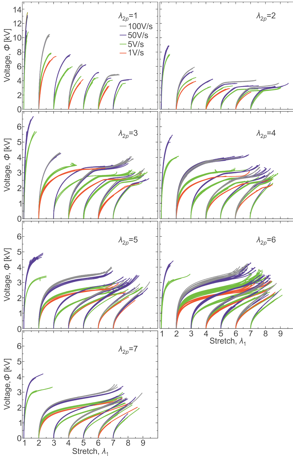
Fig. 3 The experimentally recorded voltage-stretch curves for clamped membranes in various states of prestretches \{\lambda_{1p}, \lambda_{2p}\} at different voltage ramp rates.
