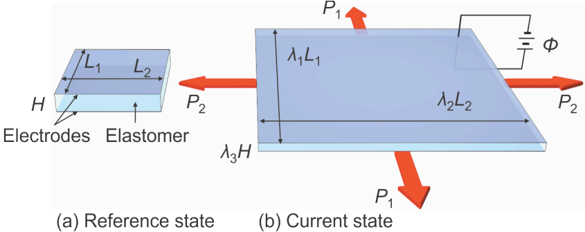
Fig. 1 A membrane of a dielectric elastomer, sandwiched between two compliant electrodes, is at (a) the reference state and (b) a current state.
