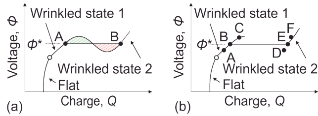
Fig. 8 Wrinkled-to-wrinkled transition. The membrane exhibits a continuous transition from the flat state to the wrinkled state, and then exhibits a discontinuous transition from the wrinkled state with a large wavelength to that with a small wavelength. (a) An elastic model is employed. The critical voltage \phi^* is at the level which makes two shaded regions have the equal area. (b) A viscoelastic model is employed. The critical voltage \phi^* is at the level which make wrinkled state 1 (with large wavelength) and wrinkled state 2 (with small wavelength) have same energy density.
