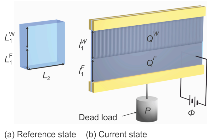
Fig. B1 During a discontinuous phase transition, the flat and wrinkled regions can coexist. (a) In the reference state, the flat and wrinkled regions are of lengths L_1^F and L_1^W , respectively. (b) In the current state, the flat and wrinkled regions are of lengths l_1^F and l_1^W and charges Q^F and Q^W .
