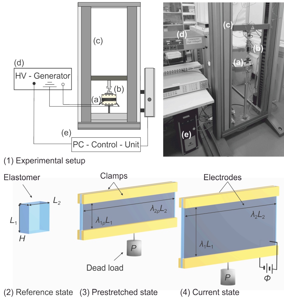
Fig. 2 (1) The experimental setup consists of a clamped dielectric elastomer membrane (a), an external strain gauge (b), a frame structure (c), and a high voltage generator (d), which can be controlled by a PC (e). The dielectric elastomer membrane can be fabricated as follows. (2) The membrane is stress free. (3) The membrane is constrained by rigid clamps and subject to a force P , and then coated with compliant electrodes on both surfaces. The membrane has stretches \lambda_{1p} and \lambda_{2p} . (4) The membrane is subject to a voltage \Phi , and expands in the vertical direction. The membrane has stretches \lambda_1 and \lambda_2 .
