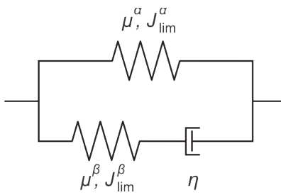
Fig. 4 A model of viscoelasticity for a membrane of a dielectric elastomer, which combines two units. One is an elastic spring ( \square ); the other is an elastic spring ( \square ) in series with a viscous dashpot.
