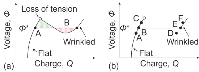
Fig. 6 The membrane exhibits a discontinuous transition from the flat state to the wrinkled state, and the flat and wrinkled regions can coexist at \phi^* . (a) An elastic model is employed. The critical voltage \phi^* is at the level which makes two shaded regions have the equal area. (b) A viscoelastic model is employed. The critical voltage \phi^* is at the level which makes the flat and wrinkled states have the same energy density.
