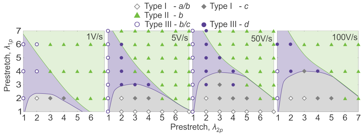
Fig. 12 The clamped membrane of a dielectric elastomer shows different kinds of behavior, depending on pre-stretches and voltage ramp rates. The theory predicts that the membrane exhibits Type I transition in the grey area, a Type II transition in the green area and a Type III transition in the blue area. The diamonds, triangles and circles corresponds to the dominant experimental observations of expected electromechanical behavior sketched in Fig. 11.
