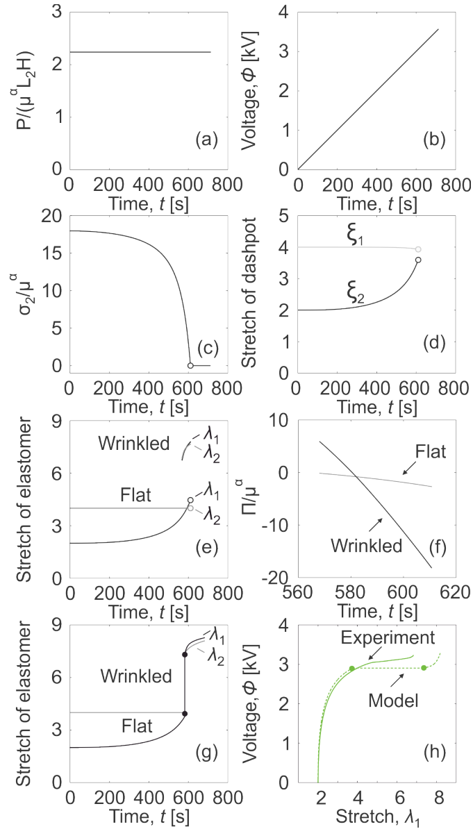
Fig. 7 Evolution and snap in the membrane of pre-stretches {2,4} at a voltage ramp rate of 5 V/s. (a) The membrane is subject to a constant load in the vertical direction. (b) Voltage increases at a ramp rate of 5 V/s. (c) Horizontal tensile stress reduces as the voltage increases. At t = 613 s, the horizontal tensile stress vanishes indicated by an open circle. (d) Evolution of the dashpot deformation. (e) Evolution of the elastomer deformation. When t = 568 s, another wrinkled state of equilibrium exists. (f) Energy densities of the flat and wrinkled states. When t = 582 s, the two states have the same energy densities. (g) Evolution of the elastomer deformation. The snap through instability may occur at t = 582 s. (h) Voltage-stretch curves. The solid curve represents the experimental data, while the dashed curve represents the theoretical predictions. At a certain voltage, the membrane transforms from the flat state to the wrinkled state, accompanied with a sudden snap in the vertical displacement indicated by filled circles.
