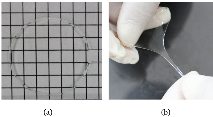
Figure 1. A polyacrylamide hydrogel containing lithium chloride. (a) The hydrogel is highly transparent. (b) The hydrogel is highly stretchable.
