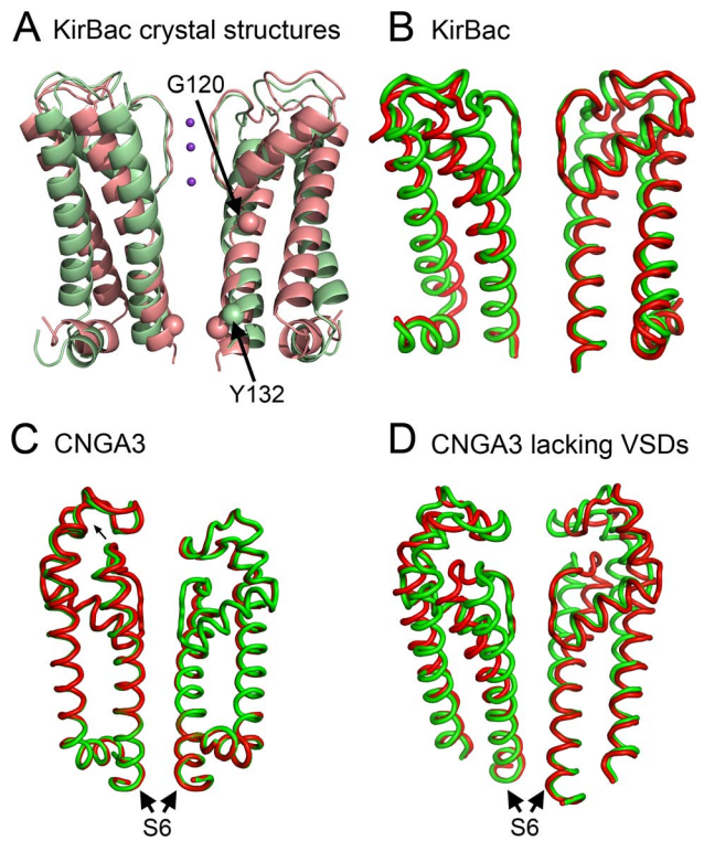
Figure 5. Motion I of CNGA3 appears to describe channel gating.
