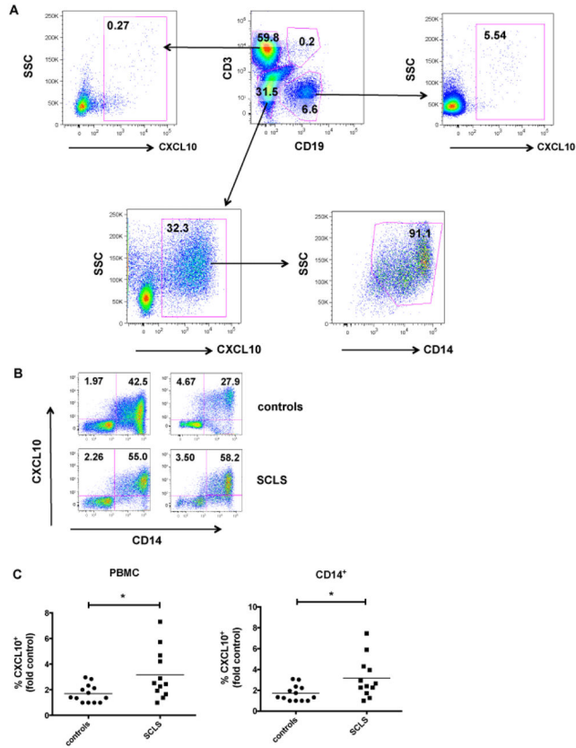
Figure 4. Abnormal IFN \gamma -induced CXCL10 production by PBMCs in SCLS. PBMCs were incubated with IFN \gamma and analyzed for CXCL10 production by flow cytometry. (A) Percentages of CXCL10+ cells among T lymphocytes (CD3+), B lymphocytes (CD19+), and monocyte (CD14+) populations from a representative healthy subject. (B–C) Representative flow plots (B) and analysis of CXCL10+ PBMCs and monocytes from SCLS subjects (n = 12) and healthy subjects (n = 14), presented as the fold control of the lowest value from a healthy donor for each individual experiment, set as ‘1’. *P = 0.02, unpaired t test.
