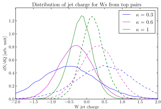
FIG. 4. Sum of jet charges of the two non b -jets in semi-leptonic t\bar{t} events with a positively (solid) or negatively (dashed) charged lepton.
