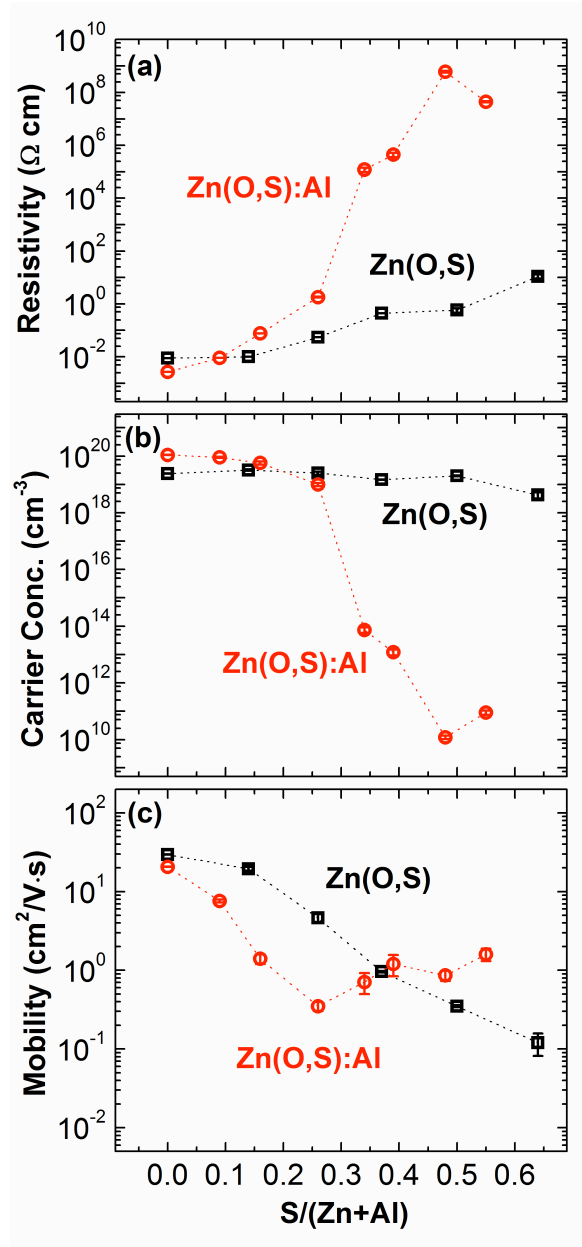
Fig. 3. Plots of (a) resistivity, (b) electron carrier concentration, and (c) carrier mobility vs. S/(Zn+Al) for Zn(O,S) (black) and Zn(O,S):Al (red) films.
