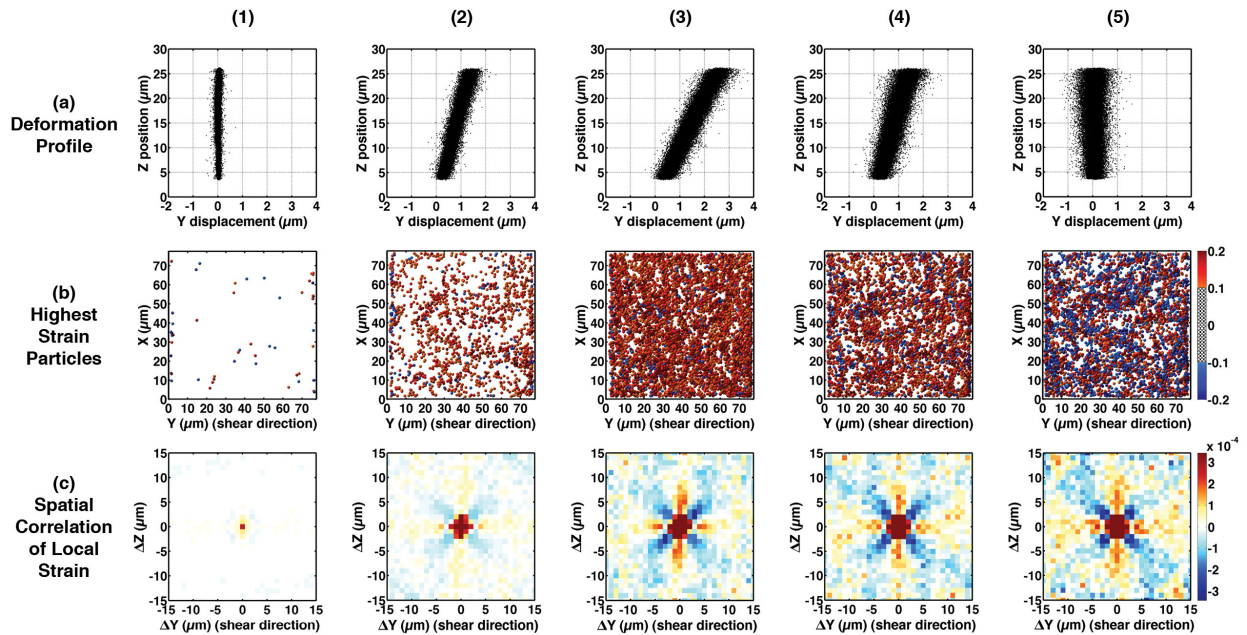
FIG. 6. (Color online) Evolution of strain and strain correlations in the colloidal glass during a shear experiment. The time and macroscopic strain corresponding to columns (1)-(5) are indicated in Figure 5c. Row (a): The deformation profiles. Row (b): Top-view reconstructions showing only those particles with individual strain |\epsilon_{yz}| > 0.1 , colored according to their strain. On strain reversal, some of the regions of particles that acquire a high positive strain (red color) return to a low-strain configuration and disappear from the reconstruction; others experience an irreversible local deformation and remain in a high-strain state at the end of the experiment. These are compensated for by other regions that deform in the opposite direction (blue color), so that at the end the average strain is zero at time (5). Row (c): y - z plane cross-sections of \epsilon_{yz} spatial autocorrelations, showing the evolution of the four-fold pattern that is the signature of Eshelby inclusions active in the material.
