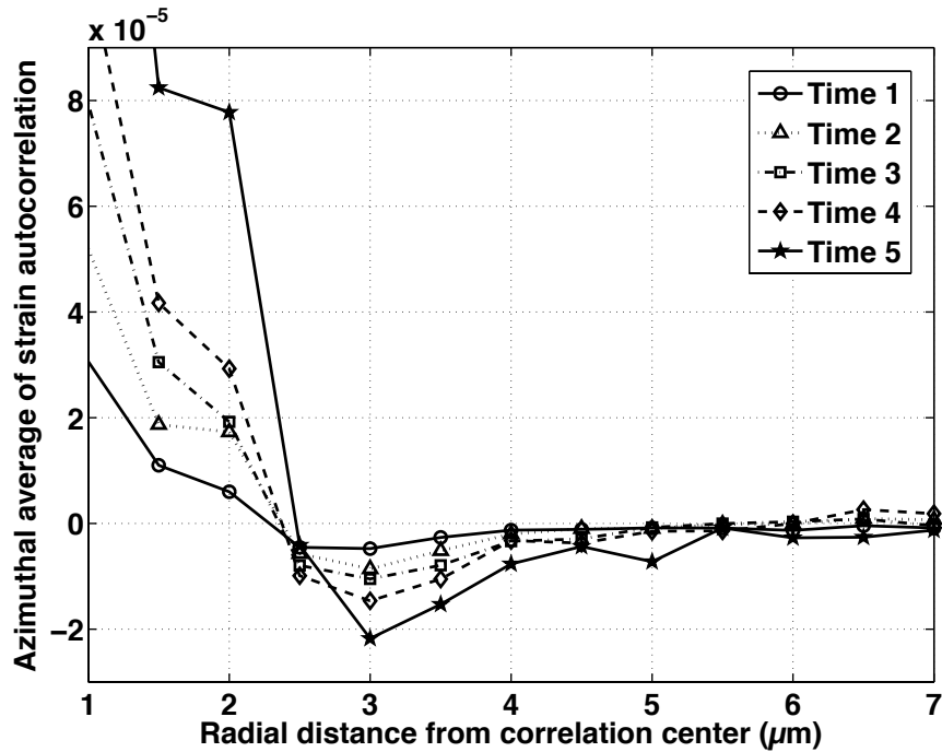
FIG. 10. Azimuthal average of the y - z spatial strain field autocorrelation in the y - z plane versus radial distance from the correlation center for both the sheared and quiescent samples (top and bottom, respectively). The times refer to Figure 5(c). Note that the vertical axis for the sheared plot is 10x that of the quiescent plot; this is due to the slower evolution of local strain in the quiescent sample.
