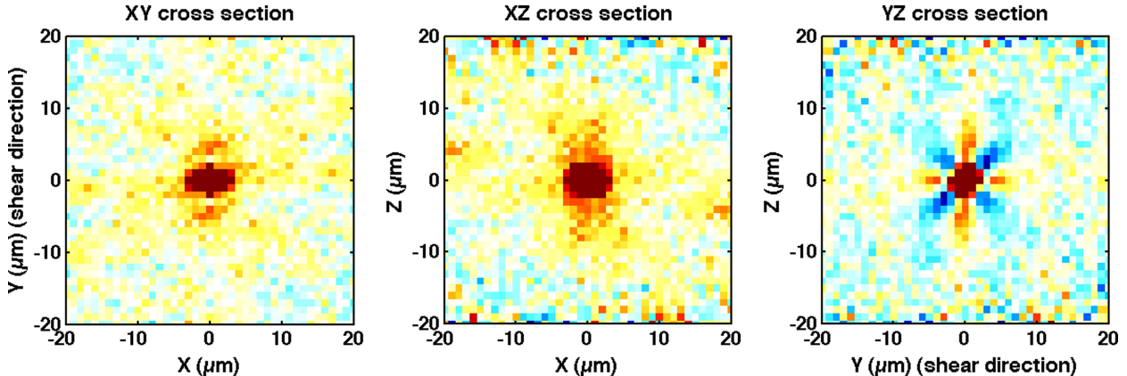
FIG. 9. (Color online) (a) x - y , (b) x - z , and (c) y - z plots of the spatial autocorrelations of the \epsilon_{yz} strain field at maximum applied strain ( \gamma_{max} = 10.0\% , t = 5040 seconds), revealing the characteristic 3D structure of an Eshelby inclusion (shown in Figure 1).
