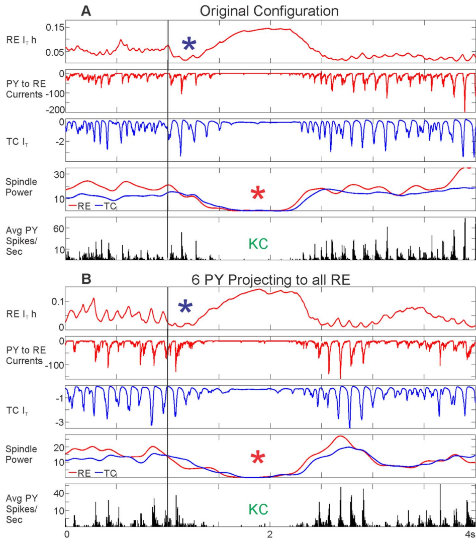
Figure 10. Inducing KCs by abruptly increasing RE I_T inactivation (RE I_T h). A, In the original configuration and B, in the 6 PY neurons projecting to all RE neurons configuration, RE I_T h is scaled to 40% of its original value (purple asterisks) at 1 s (vertical black line). In other words, the proportion of deactivated I_T channels is abruptly decreased. In both cases, this drop in RE I_T h leads to a decrease in PY to RE currents and TC I_T , as well as a drop in RE and TC spindling (red asterisks), which ultimately leads to a KC, as indicated by decreased PY spiking (“KC”). doi:10.1371/journal.pcbi.1003855.g010
