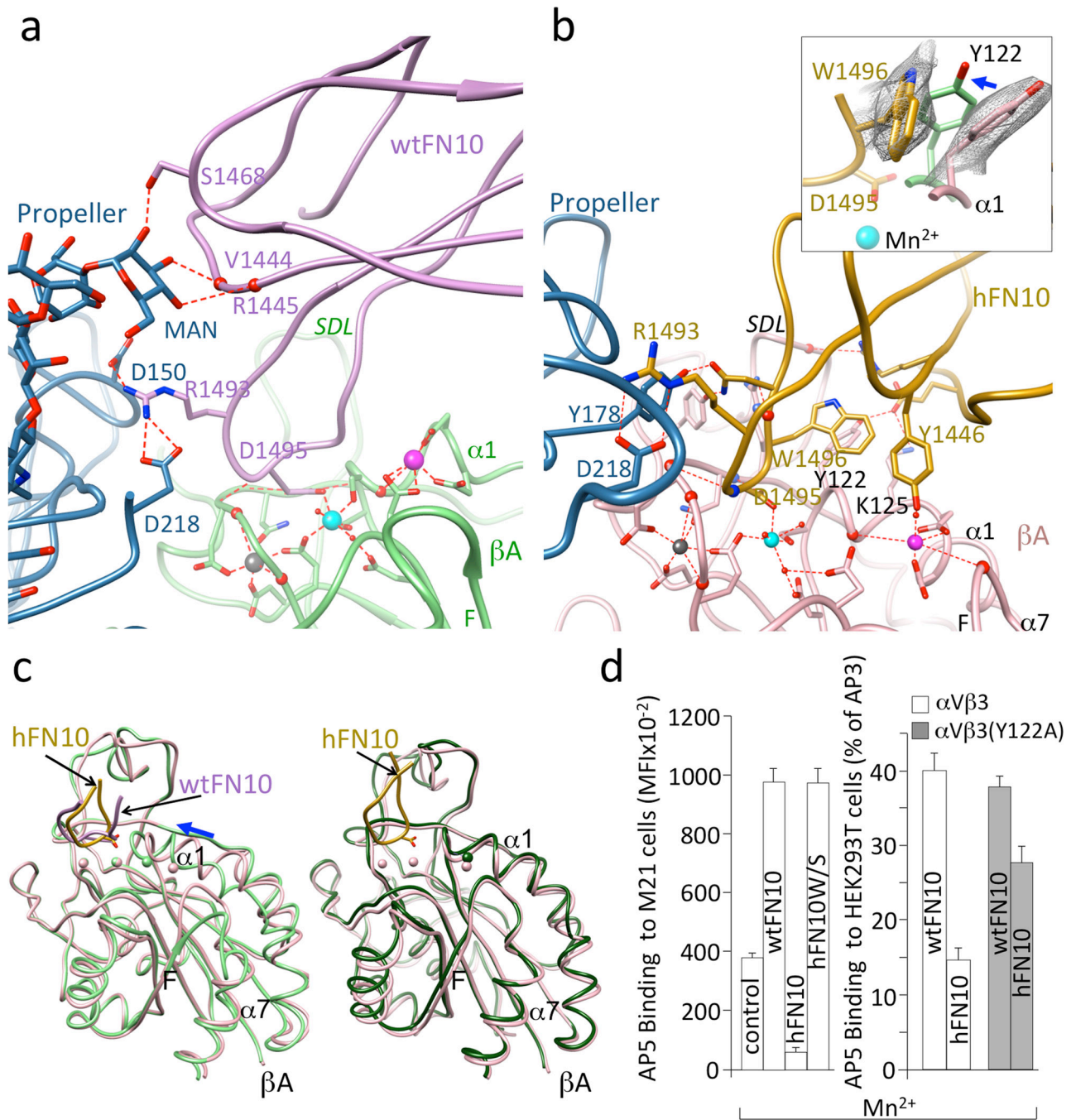
Figure 3. \alpha V \beta 3-FN10 interfaces, conformational changes and structure validation
