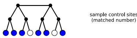
D correlation between site pairs compared to independent evolution
