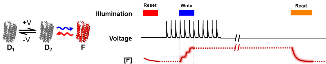
Figure 3-1. Classes of voltage indicators. (a) In a real-time voltage reporter, the population in a fluorescent state, F , is a function of membrane voltage, regardless of illumination. (b) In a sample and hold voltage sensor, voltage establishes a D_1 \rightleftharpoons D_2 equilibrium and a write pulse establishes a rapid D_2 \rightleftharpoons F equilibrium. Thus the population of F tracks the membrane voltage. The population of F is frozen at the end of the write pulse. (c) In a light-gated voltage integrator, voltage establishes a D_1 \rightleftharpoons D_2 equilibrium and a write pulse drives the unidirectional D_2 \rightarrow F transition. Thus the population of F accumulates in a voltage-dependent manner. The population of F is frozen at the end of the write pulse. In both types of Flash Memory sensor, the population of F persists in the dark and is later probed via a read pulse that elicits fluorescence.
