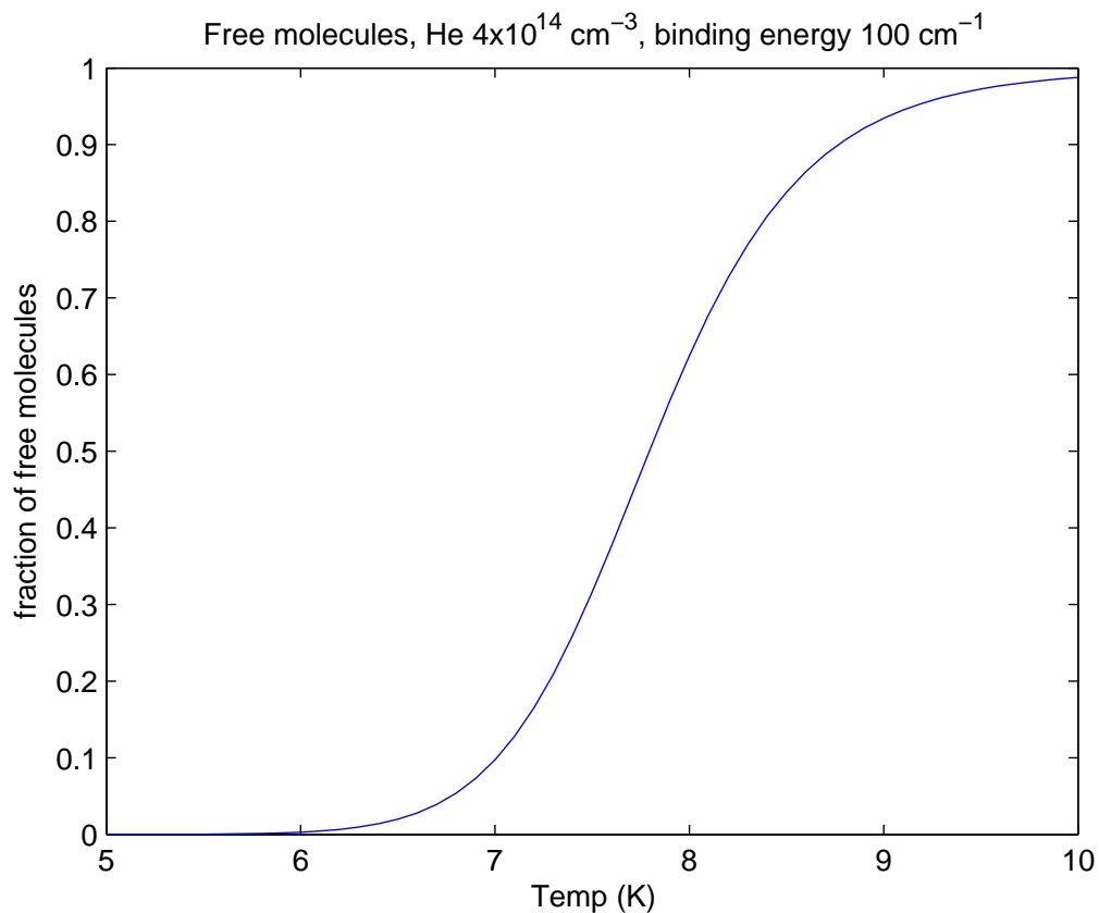
Figure 3.1: Fraction of free molecules in equilibrium as a function of temperature for a binding energy of 100\text{ cm}^{-1} and helium density of 4\times 10^{14}\text{ cm}^{-3} . At a typical cell temperature of 7 K, the majority of molecules are clustered in equilibrium.
