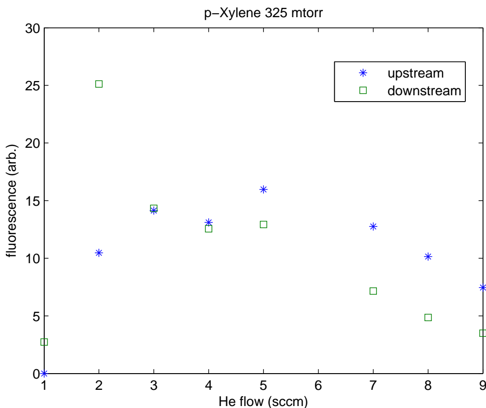
Figure A.3: Fluorescence of the electronic origin of p -Xylene vs helium buffer gas flow.
