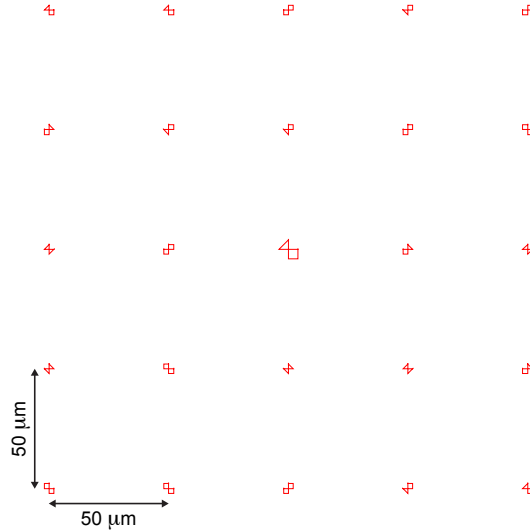
Figure A.4: EBL defined alignment marks in a 50 \mu\text{m} by 50 \mu\text{m} grid. Nanowires are located relative to these alignment marks by using optical microscopes or SEMs. The permutation of different alignment marks ensures that images of nanowires are not incorrectly overlaid on the CAD file during device design.
