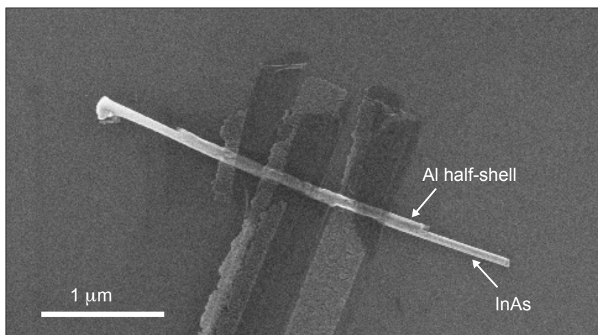
Figure A.11: SEM micrograph of an epitaxial half-shell nanowire, post etch. The nanowire is held down by two evaporated Al contacts. Debris on the chip are most likely due to the redeposition of \text{SiO}_2 during ion milling.
