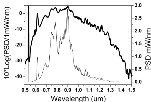
Fig. 3. Output spectrum of the 1 GHz laser used as the source comb for the visible wavelength astro-comb. The large peak at 532 nm is residual power from the pump laser.
