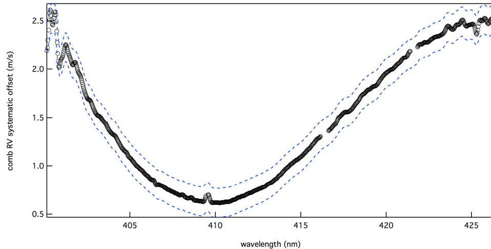
Fig. 7. Offset of recovered astro-comb line center caused by misalignment of filter cavity transmission maximum and the source comb lines as measured by the TRES spectrograph (black circles). Error bars at \pm 15 cm/s on the recovered offset correspond to the uncertainty of the laser diode frequency used to lock the filter cavity and astro-comb (blue dotted lines). Breaks in the data set at 417 nm and again at 422 nm correspond to transitions between spectrograph orders as recovered from the CCD. The glitch at 408 nm is caused by amplitude to phase conversion by slight saturation of the CCD by the laser diode. Increased fluctuation in the trace above 424 nm and below 402 nm is due to the reduced signal to noise ratio at the edges of the astro-comb spectrum. The offset of recovered astro-comb lines has been low pass filtered to remove oscillations caused by mild etalon effects from the mirror substrates, see text above.
