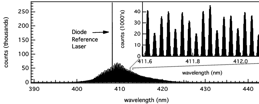
Fig. 6. Extracted one dimensional spectrum of full astro-comb spectrum. The FWHM of the spectrum is approximately 10 nm, with approximately 50,000 peak counts in 10 seconds on the spectrograph. Inset: example of filtered comb lines with mode spacing of 51 GHz. The diode reference laser is used for characterization of the filter cavity transmission profile described in the text.
