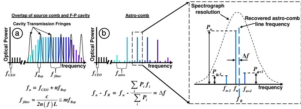
Fig. 1. Description of an astro-comb in the frequency domain. (a) Frequency-doubled source comb lines and analytic description of the optical spectrum in terms of the repetition rate, f_{rep} , and the carrier envelope offset frequency, f_{CEO} , of the underlying Ti:Sapphire laser. The frequency doubled spectrum is multiplied by the transmission function of the Fabry-Perot cavity, filtering the source comb spectrum which becomes the astro-comb spectrum shown in graph (b). The free spectral range of the transmission resonances of the filter cavity, f_{filter} , is ideally an integer multiple of the repetition rate of the source laser. However due to dispersion from air and mirror reflections, f_{filter} will generally be a function of frequency. In this example the integer m = 4 (typically m = 20-50 with our 1 GHz repetition rate laser) such that in (b) every 4th line (referred to as an astro-comb line) is fully transmitted. Because the spectrograph resolution ( \sim 15 GHz) is generally larger than the repetition rate of the source comb, finite suppression of the source comb modes closest every astro-comb line results in a power weighted average frequency, f_R , to be reported by the spectrograph. The difference \Delta f must be recovered to realize the full accuracy of the astro-comb.
