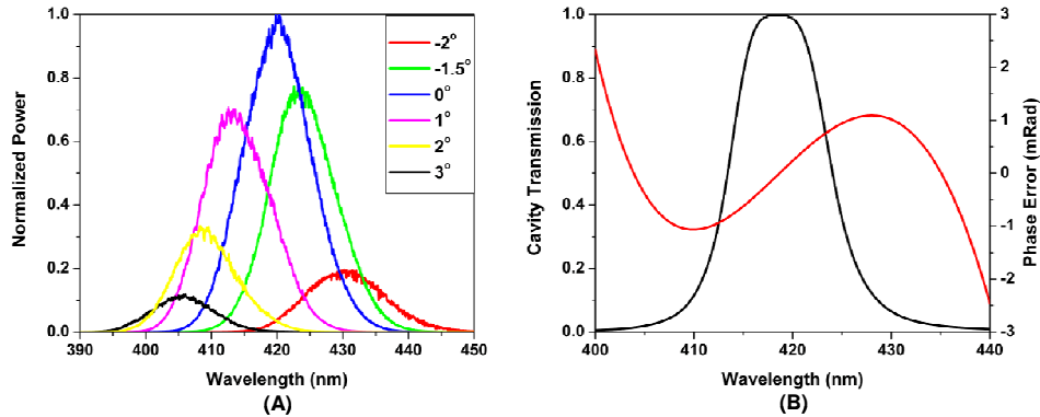
Fig. 4. (A) Measured optical spectra of the visible wavelength astro-comb, after the Fabry-Perot cavity filter, for several angles of the BBO crystal relative to the IR source comb beam. Integrated power for the central spectrum is 25 \mu\text{W} ( \sim 25 nW per astro-comb line). Filtered mode spacing is 22 GHz. (B) Calculated characteristics of the Fabry-Perot cavity filter using dispersion-optimized dielectric Bragg reflectors. Round-trip dispersion due to reflection from the Fabry-Perot cavity mirrors is plotted on the right axis, and cavity transmission for an input spectrum centered at 420 nm is plotted on the left axis taking into account air dispersion as well as mirror dispersion and reflectivity.
