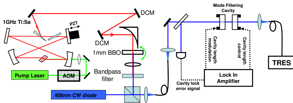
Fig. 2. Layout for visible wavelength astro-comb. Output from an octave-spanning 1 GHz Ti:Sapphire laser frequency comb is pre-chirped using two Dispersion Compensating Mirrors (DCM) and focused with an off-axis parabolic mirror into a BBO crystal. Single mode fiber between the Ti:Sapphire laser and the Fabry-Perot cavity filter ensures that the spatial profile of the beam entering the cavity is of lowest order ( TEM_{00} ), giving the best possible suppression of transmission by higher order transverse modes. A 408 nm external cavity diode laser allows for identification of the desired Fabry-Perot cavity length as well as side-mode suppression estimation. TRES – Tillinghast Reflector Echelle Spectrograph, AOM – acousto-optic modulator, PZT – piezo electric transducer.
