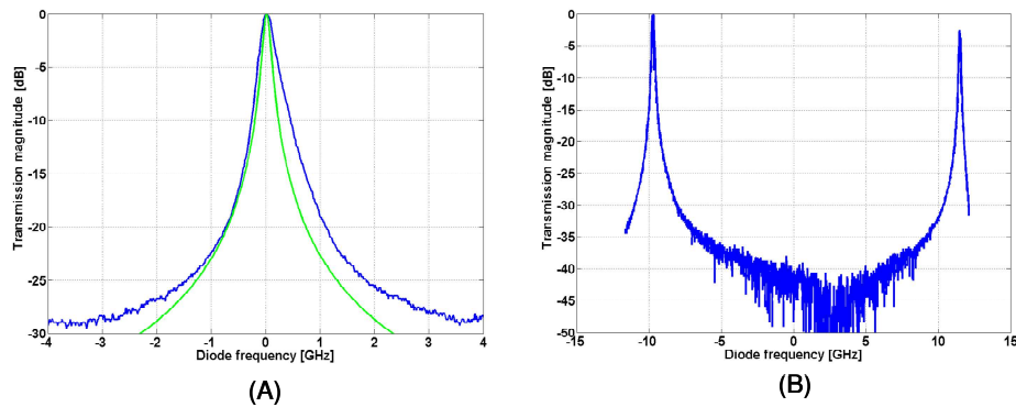
Fig. 5. Transmission of the Fabry-Perot cavity filter measured with a swept frequency laser diode. (A) Comparing measured transmission (blue) and calculated transmission assuming R = 98.2\% and a free spectral range of 22 GHz (green) shows the asymmetric observed line shape. Coupling of the diode laser into the cavity is identical to that of the frequency comb. (B) No higher order peaks are visible in a sweep spanning the full 22 GHz free spectral range.
