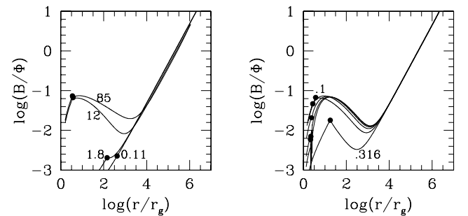
Figure 5. Variation with radius of the Bernoulli parameter \mathcal{B} (equation 13), normalized by the gravitational potential, for the four solutions shown in Fig. 1 (left-hand panel) and the six solutions shown in Fig. 3 (right-hand panel). The solid dots indicate the positions of the sonic radii. Curves are labelled by their values of \mathcal{L} in the left-hand panel and \alpha in the right-hand panel.
