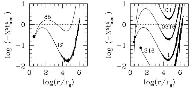
Figure 6. Left: variation with radius of the quantity -N^2 t_{\text{acc}}^2 , which is a measure of convective instability, for two of the four solutions shown in Fig. 1. (The other two are below the bottom of the plot.) The dotted line indicates our nominal threshold for becoming convection-dominated. The more rapidly spinning solution ( \mathcal{L} = 85 ) goes above the dotted line over a range of radius, and we expect it to become a CDAF in this zone. The less rapidly rotating solution ( \mathcal{L} = 12 ) lies below the dotted line and probably will not become a CDAF. Right: corresponding results for the solutions shown in Fig. 3. The two solutions with \alpha = 0.316 and 0.1 lie below the dotted line and will not be convection-dominated, while the solutions with smaller values of \alpha are expected to become CDAFs. Note that none of the curves in the two panels extends inside the sonic radius. This is because we have assumed the flow to be inviscid once it becomes supersonic. The specific entropy is then constant (Subsection 2.2) and N^2 = 0 .
