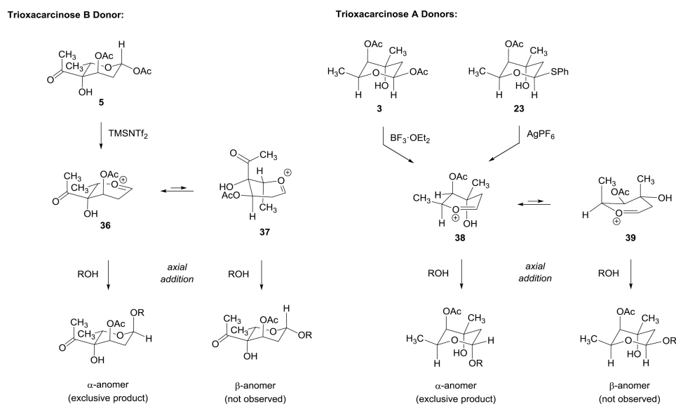
Figure 6. Rationalizations of the stereochemical outcome of glycosylation reactions with trioxacarcinose A and B donors
