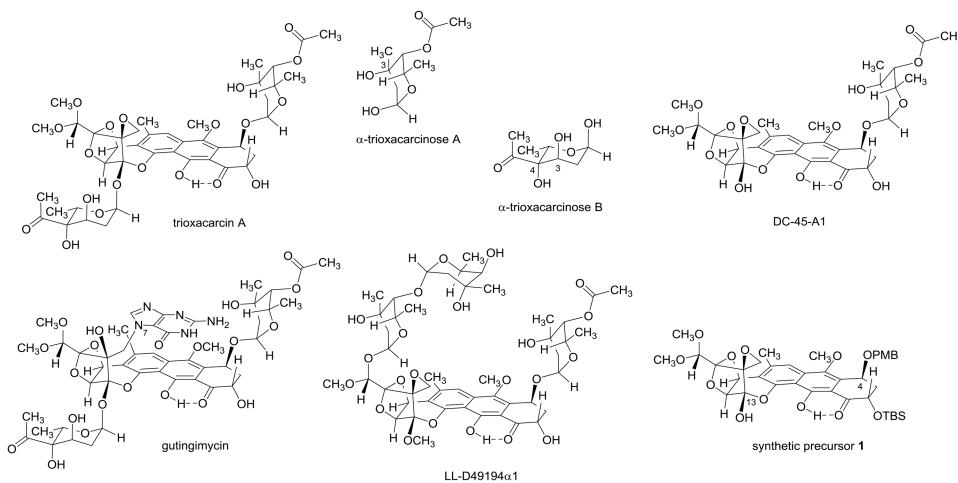
Figure 1. Trioxacarcin A and Structural Relatives
