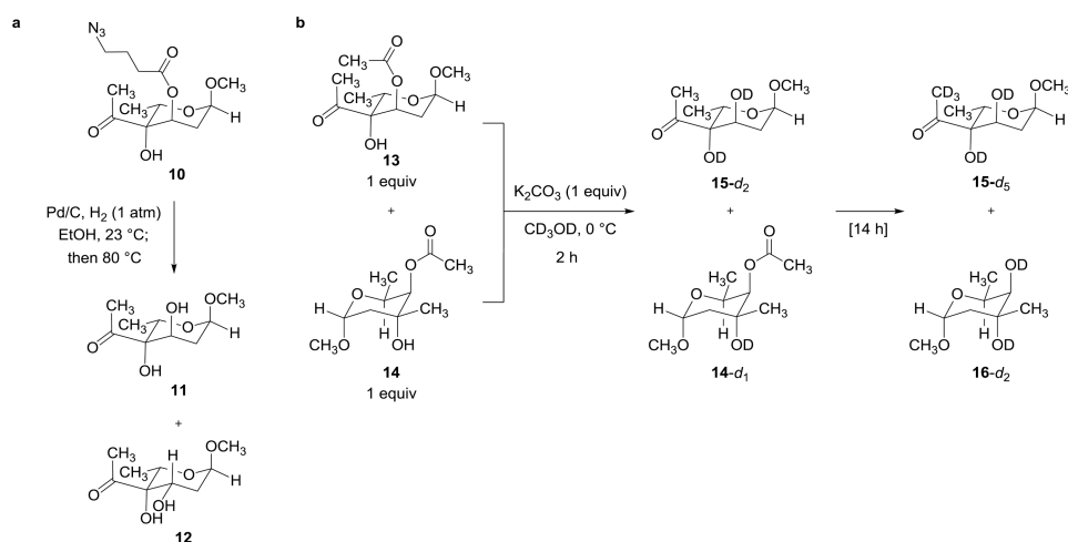
Figure 3. Model studies leading to selection of O -acetyl for protection of the 3-hydroxyl group of trioxacarcinose B
