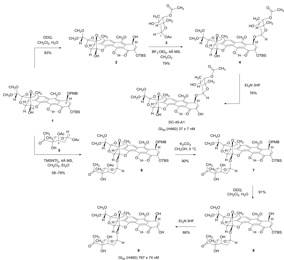
Figure 2. Syntheses of DC-45-A1 and the trioxacarcinose B-containing monoglycoside 9 Stereoselective glycosylation reactions enabled preparation of monoglycosides containing either trioxacarcinose A or B residues in sequences of three and four steps, respectively. Importantly, both glycosidations preserve the spirocyclic epoxide function.
