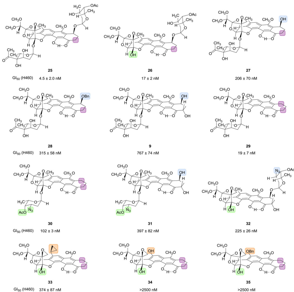
Figure 5. Fully synthetic trioxacarcin analogs
