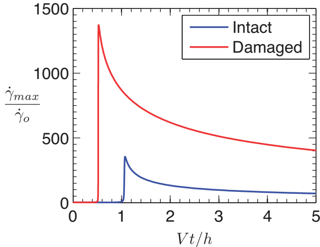
Figure 12. Gouge dilatancy: A plot showing how the maximum strain rate \dot{\gamma}_{max} evolves for the path-averaged parameters modeling an intact and a damaged material, for V = 1 m/s and h = 0.5 mm. As predicted by the linear stability analysis there is an initial transient of intense strain rate localization followed by decay to homogeneous straining. In contrast with the frictional strengthening case, the damaged material shows more intense localization.
