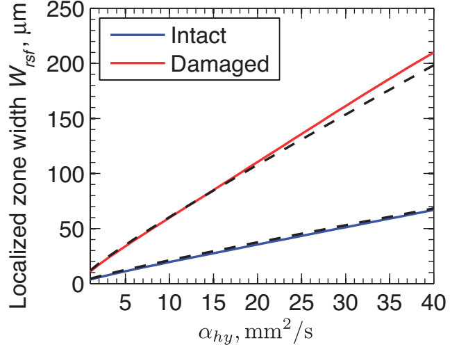
Figure 6. Rate-strengthening friction: A plot showing how the localized zone thickness W_{rsf} changes with \alpha_{hy} for the path-averaged parameters modeling an intact material and a damaged material given in Table 1, a slip rate V = 1 m/s and gouge layer thickness h = 1 mm. This parameter sweep allows us to vary the dimensionless parameter D_{hy} while the other two dimensionless parameters D_{th} and z remain unchanged. The black dashed lines show the fitting formula given in equation (31). Larger values of \alpha_{hy} lead to wider localized zones. The deviation at large values of \alpha_{hy} for the damaged parameter set is due to W_{rsf} becoming comparable to h .
