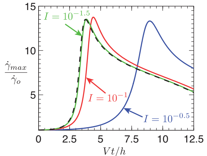
Figure 18. Rate-strengthening friction: A plot showing how maximum strain rate evolves in the inertial model for I = 10^{-0.5} , 10^{-1} and 10^{-1.5} . This plot was created using the nominal parameters modeling a damaged material, h = 0.5 mm and V = 1 m/s. For comparison the solution when mechanical equilibrium is assumed is shown by the dashed black line. For the lowest value of I the inertial and equilibrium solutions agree almost exactly, while for the larger values we see deviation away from the equilibrium solution.
