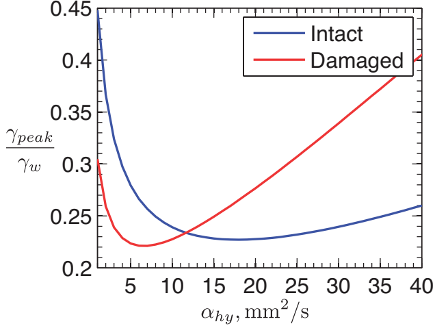
Figure 9. Rate-strengthening friction: A plot showing how the nominal strain at which peak localization occurs varies with \alpha_{hy} . These simulations were produced using the path-averaged parameters for an intact and a damaged material, V = 1 m/s and h = 1 mm. For low values of \alpha_{hy} , corresponding to localized zone thicknesses that are much smaller than the gouge layer thickness, the critical strain is a decreasing function of \alpha_{hy} . For both parameter sets \gamma_{peak} reaches a minimum before increasing at large values of \alpha_{hy} .
