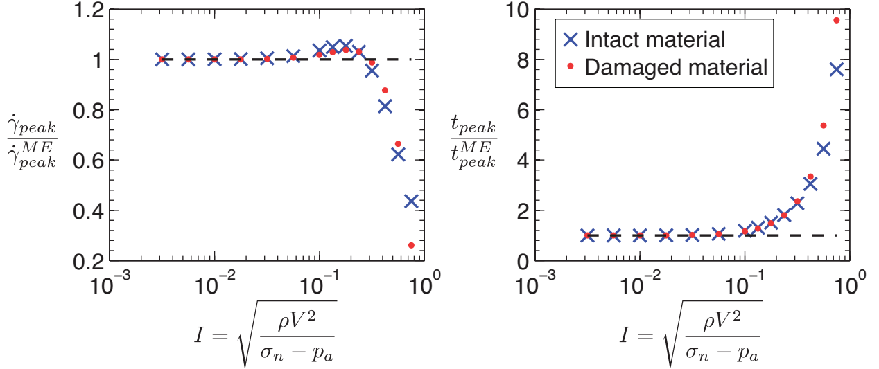
Figure 19. Rate-strengthening friction: A plot showing how the peak strain rate \dot{\gamma}_{peak} and time t_{peak} at which this peak strain occurs vary with I for the nominal parameters modeling intact and damaged material, a gouge layer thickness h = 0.5 mm, and a slip rate V = 1 m/s. To allow easy comparison between the two parameter sets all values of \dot{\gamma}_{peak} and t_{peak} are normalized by the values found when mechanical equilibrium is assumed. These mechanical equilibrium values are indicated by a superscript ME . Above I = 10^{-1} inertial effects become important and the two models diverge. Inertial effects lead to two key differences. The value of \dot{\gamma}_{peak} is decreased, which corresponds to a wider localized zone; the time t_{peak} at which peak localization occurs is larger indicating that the localized zone takes longer to develop.
