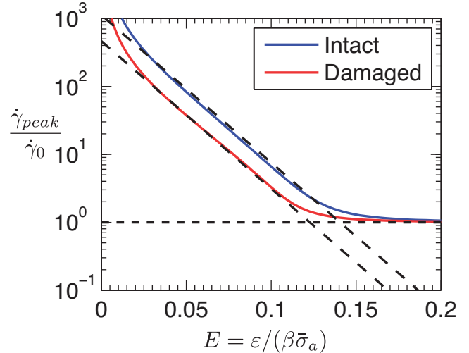
Figure 13. Gouge dilatancy: A plot showing how the peak strain rate \dot{\gamma}_{peak} depends on the dimensionless parameter E = \epsilon/(\beta\bar{\sigma}_a) for the dilatancy only system using the path-averaged parameters modeling an intact and a damaged material, V = 1 m/s and h = 0.5 mm. For both parameter sets we observe larger peak strain rates for smaller values of E , corresponding to narrower localized shear zones. For all but the smallest values of E our results are well described by equation (47), and for each parameter set this formula is shown by the dashed black line.
