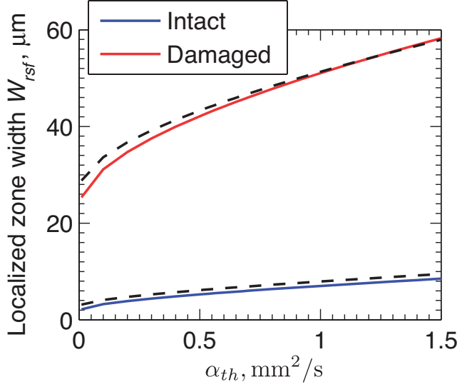
Figure 5. Rate-strengthening friction: A plot showing how the localized zone thickness W_{rsf} changes with \alpha_{th} for the path-averaged parameters modeling an intact material and a damaged material given in Table 1, a slip rate V = 1 m/s and gouge layer thickness h = 1 mm. This parameter sweep allows us to vary the dimensionless parameter D_{th} while the other two dimensionless parameters D_{hy} and z remain unchanged. The black dashed lines show the fitting formula given in equation (31). Larger values of \alpha_{th} lead to wider localized zones.
