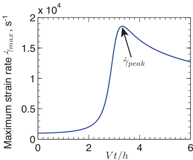
Figure 2. Rate-strengthening friction: The blue curve shows the evolution of the maximum strain rate \dot{\gamma}_{max} within the gouge layer for the path-averaged parameters modeling a damaged material, V = 1 m/s and h = 1 mm. The maximum strain rate grows indicating that straining is localizing within the gouge layer. After a finite amount of slip the peak strain rate begins to decay indicating that the localized zone is thickening. This thickening occurs whenever both \alpha_{th} and \alpha_{hy} are non-zero. We define the peak strain rate \dot{\gamma}_{peak} to be the largest value of \dot{\gamma}_{max} .
