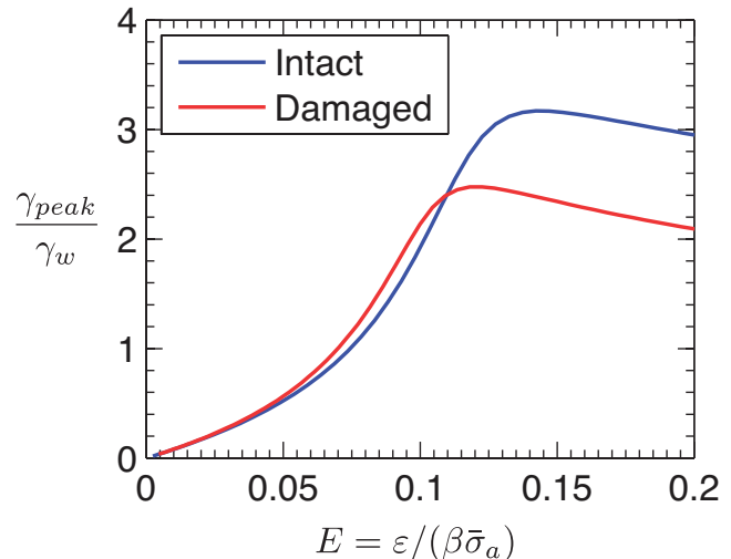
Figure 15. Gouge dilatancy: A plot showing how \gamma_{peak} , the strain at which peak localization occurs, depends on E . These simulations were done using the path-averaged parameters for an intact and damaged material, V = 1 m/s and h = 0.5 mm. Our results show that when E is small enough that transient strain rate localization occurs \gamma_{peak} is an increasing function of E , with small values of E leading to small values of \gamma_{peak} . This means that the most intense localized zones develop very rapidly. Very little difference is observed between the two parameter sets, which can be explained by noting that \gamma_{peak} is relatively insensitive to changes in L_{thd} , as shown in Figure 16.
