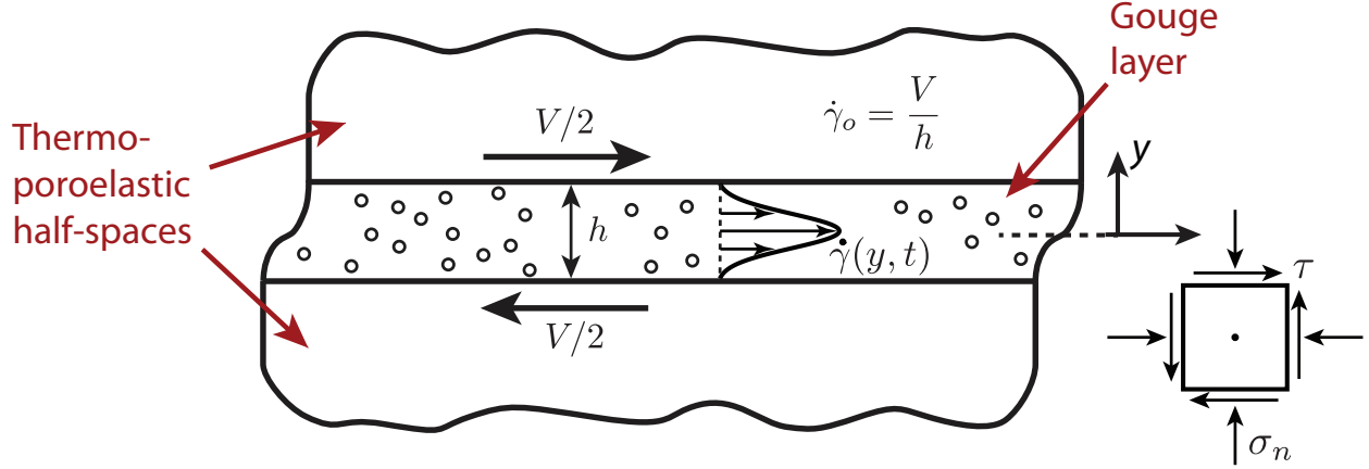
Figure 1. A sketch showing the system we are modeling. A gouge layer with a finite thickness h is sheared between two rigid poroelastic half-spaces that are moved relative to each other at a slip rate V . This leads to a nominal strain rate within the gouge layer \dot{\gamma}_o = V/h . The strain rate \dot{\gamma}(y, t) will localize within the gouge layer, as shown by the Gaussian strain rate profile sketched within the gouge layer. The width W of the zone of localized straining is then estimated as twice the root mean square width of the Gaussian.
