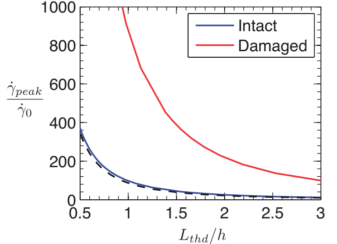
Figure 14. Gouge dilatancy: A plot showing how the peak strain rate \dot{\gamma}_{peak} depends on the ratio of the thermal diffusion distance L_{thd} = 2\pi\sqrt{\alpha_{th}t_w} , where t_w is the characteristic weakening time for thermal pressurization, and the gouge layer thickness h . These simulations were produced using the path-averaged parameters modeling an intact and a damaged material, V = 1 m/s and h = 0.5 mm. Larger values of L_{thd} , corresponding to more efficient thermal diffusion, lead to lower peak strain rates and thus wider localized zones. The simulations are well fit by the formula given in equation (47), and this curve is shown by the dashed black line. No line is shown for the damaged parameters since the value of E is sufficiently small that equation (47) is no longer accurate.
