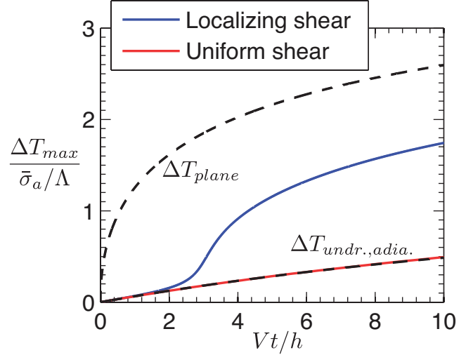
Figure 11. Rate-strengthening friction: A plot showing how the maximum temperature rise, \Delta T_{max} = T_{max} - T_a , in the gouge layer evolves for localized and uniform shear using the path-averaged parameters for a damaged material, h = 1 mm and V = 1 m/s. The initial behavior, before localization and diffusion become important, is well described by the undrained adiabatic solution of Lachenbruch [1980] (marked \Delta T_{undr.,adia.} ). As straining localizes the frictional heating is focused into a zone much narrower than the gouge layer thickness, leading to a sharp temperature rise. After localization the localized shear solution mirrors the Mase-Smith-Rice slip on a plane solution (marked \Delta T_{plane} ), but the slip on a plane solution never provides a good approximation for maximum temperature rise.
