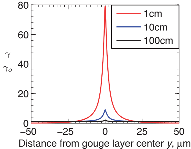
Figure 17. Gouge dilatancy: A plot of the final strain normalized by the average strain in the layer \gamma_o , for slips of 1 cm, 10 cm and 100 cm. These results were generated using the path-averaged parameters for a damaged material, V = 1 m/s, and h = 0.5 mm. We observe a decrease in strain localization with increasing slip. This can be understood by considering the transient nature of the localization; longer events will spend more time straining uniformly, and thus the effects of the transient strain rate localization will be less pronounced in the final strain profile.
