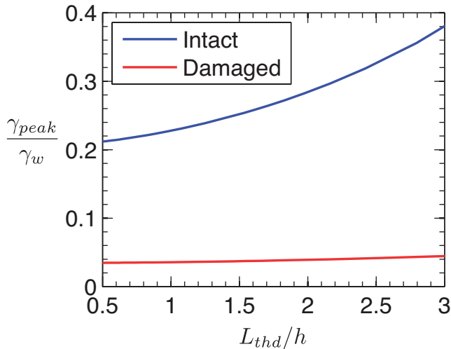
Figure 16. Gouge dilatancy: A plot showing how \gamma_{peak} , the strain at which peak localization occurs, depends on the ratio of the thermal diffusion distance L_{thd} = 2\pi\sqrt{\alpha_{th}t_w} , where t_w is the characteristic weakening time for thermal pressurization, and the gouge layer thickness h . These simulations were done using the path-averaged parameters for an intact and damaged material, V = 1 m/s and h = 0.5 mm. Our results show that \gamma_{peak} is an increasing function of L_{thd} , though when the localized zone width is much smaller than the gouge layer thickness \gamma_{peak}/\gamma_w does not depend strongly on L_{thd} .
