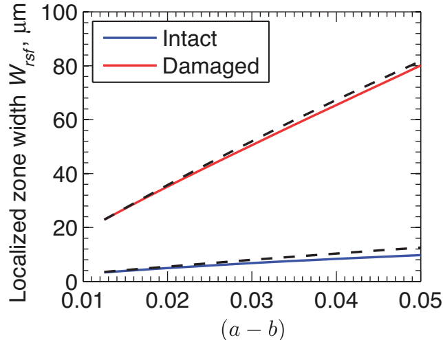
Figure 7. Rate-strengthening friction: A plot showing how the localized zone thickness W_{rsf} changes with (a-b) for the path-averaged parameters modeling an intact material and a damaged material given in Table 1, a slip rate V = 1 m/s and gouge layer thickness h = 1 mm. This parameter sweep allows us to vary the dimensionless parameter z while the other two dimensionless parameters D_{hy} and D_{th} remain unchanged. The black dashed lines show the fitting formula given in equation (31). Larger values of (a-b) lead to wider localized zones.
