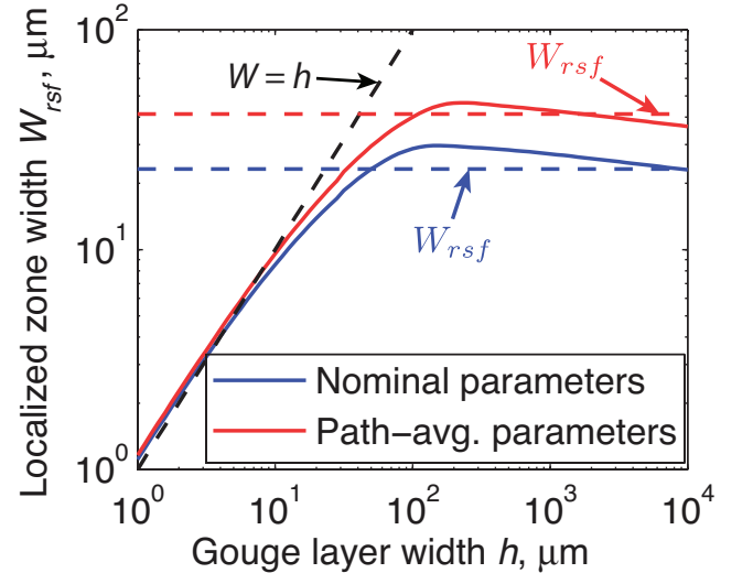
Figure 4. Rate-strengthening friction: Figure showing how the localized zone thickness W_{rsf} at peak localization depends on gouge layer thickness h . Numerical results for the path-averaged and nominal parameters for a damaged material and a slip rate of V = 1 m/s are shown by solid colored lines, with the accompanying linear stability predictions for these parameters shown by dashed colored line. For thin gouge layers we see that the localized zone thickness is equal to the gouge layer thickness, with the line W = h shown by dashed black line for guidance. When the gouge layer thickness is large the straining localizes to a width that is only weakly dependent on the gouge layer thickness. This width is in good agreement with the predictions for W_{rsf} from the linear stability analysis in Rice et al. [2013].
