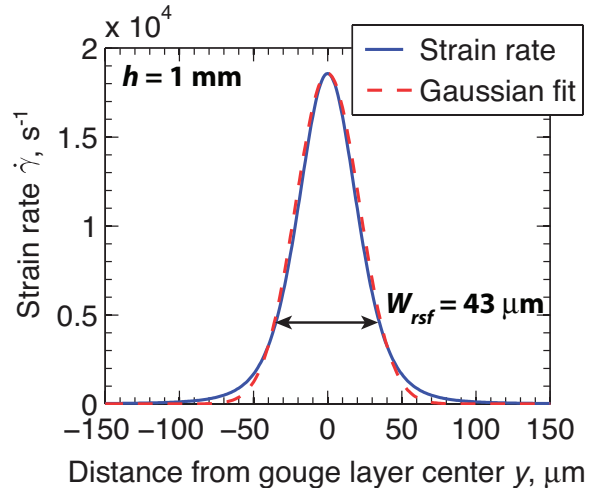
Figure 3. Rate-strengthening friction: A plot showing the strain rate profile at peak localization for the path-averaged parameters modeling a damaged material, V = 1 m/s and h = 1 mm. The numerical solution is shown in blue with the Gaussian fit defined by equation (27) shown by the red dashed line. The width W_{rsf} of the localized zone is estimated as twice the root mean square width of the Gaussian, and we find W_{rsf} = 43 \mu m.
