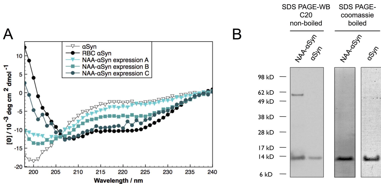
Figure 1. Variability in the folding of purified recombinant NAA- \alpha S under non-denaturing conditions. A: CD spectroscopy of bacterially expressed and purified NAA- \alpha S and \alpha S under non-denaturing conditions. No variability in the secondary structure was seen with unmodified \alpha S. In contrast, NAA- \alpha S showed batch-to-batch variability in folding of the obtained preps. B: SDS-PAGE Western blot and Coomassie stain of \alpha S and NAA- \alpha S ("expression C"). The samples were not boiled in SDS-sample buffer before gel loading for Western blotting. The NAA- \alpha S banding pattern indicates some SDS-stable tetrameric protein present in the sample, while no higher bands could be detected in non-acetylated \alpha S. For coomassie staining, the samples were boiled in sample buffer, leading to a single stainable band at 14 kDa, indicative of the high purity of the sample. doi:10.1371/journal.pone.0103727.g001
