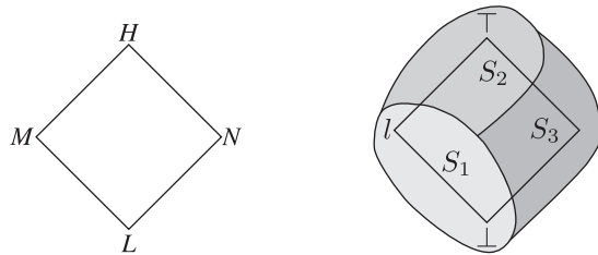
(a) 4-element Hasse diagram (b) Disjoint sets in update Figure 5: Example security lattice and disjoint sets in update
