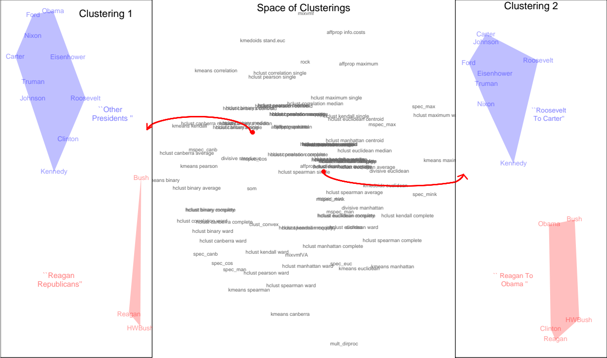
Figure 1: A Clustering Visualization: The center panel gives the space of clusterings, with each name printed representing a clustering generated by that method, and all other points in the space defined by our local cluster ensemble approach that averages nearby clusterings. Two specific clusterings (see red dots with connected arrows), each corresponding to one point in the central space, appear to the left and right; labels in the different color-coded clusters are added by hand for clarification, as is the spacing in each.
