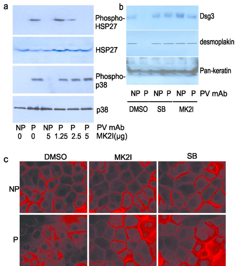
Figure 3. MK2 inhibition blocks loss of cell surface Dsg3 by pathogenic (P) PV mAb A) Pretreatment of PHEK with an MK2-specific inhibitor (MK2I) for 2 hours, then PV mAb for 2 hours, blocks phosphorylation of HSP27 but not p38 in a dose-dependent pattern. B) MK2I rescues the loss of desmosomal Dsg3 caused by P mAb. PHEK were treated with DMSO, 2μM SB202190 (p38 inhibitor) or 2.5 μg/mL MK2I for 2 hours, followed by 50 μg/ml PV mAbs (P or NP) for 6 hours. Triton X-100-insoluble fractions were immunoblotted with antibodies as indicated. Data are representative of three independent experiments. C) P but not NP mAb (as in B ) causes loss of cell surface Dsg3 (green), which is inhibited by SB202190 and MK2I. Scale bar=20μm.
