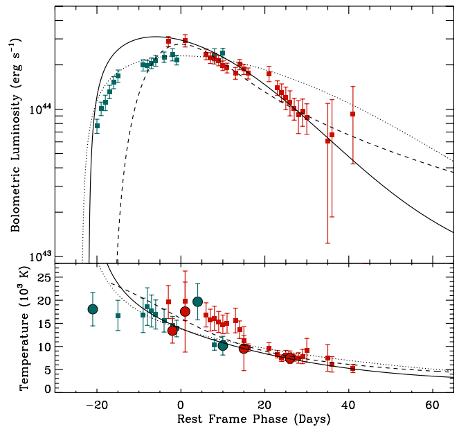
Figure 11. Top panel: combined bolometric light curve for PS1-10awh and PS1-10ky (colors and symbols as in Figure 8) fit using magnetar spin-down models (Kasen & Bildsten 2010). Different lines correspond to fits for different SN ejecta masses: M_{ej} = 1 M_{\odot} (dashed; B_{14} = 1.3 , P_{10} = 0.34 ), 5 M_{\odot} (solid; B_{14} = 3.0 , P_{10} = 0.12 ), and 10 M_{\odot} (dotted; B_{14} = 2.4 , P_{10} = 0.1 ). Bottom panel: temperature evolution plotted as in Figure 8, with the effective temperature of the magnetar spin-down models overplotted as lines as in the top panel.
