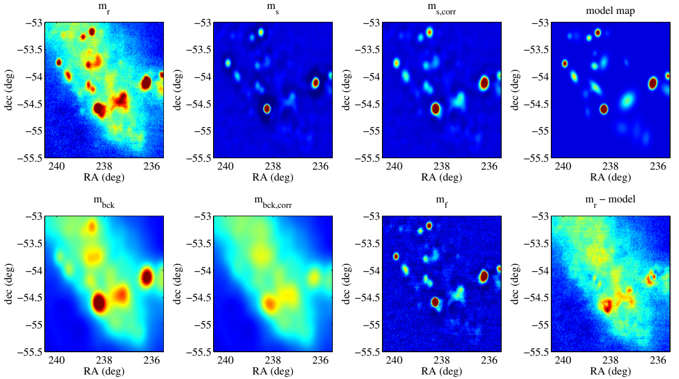
Figure 2. Source segmentation and fitting using a section of QUaD 100 GHz I data; color scale is the same in all panels and runs from -0.0035 to 0.035 MJy \text{sr}^{-1} . Top left: raw map m_r . Bottom left: initial estimate of background map m_{\text{bck}} . Top row, second column: initial background subtracted map m_s . Bottom row, second column: background map corrected for discrete source flux ( m_{\text{bck,corr}} ). Top row, third column: background subtracted map m_r using source-corrected background map m_{\text{bck,corr}} . Bottom row, third column: map used for source fitting m_r - m_{\text{bck,corr}} . Top right: model of discrete source population using fits to m_r . Bottom right: residual between model sky and input image m_r .
