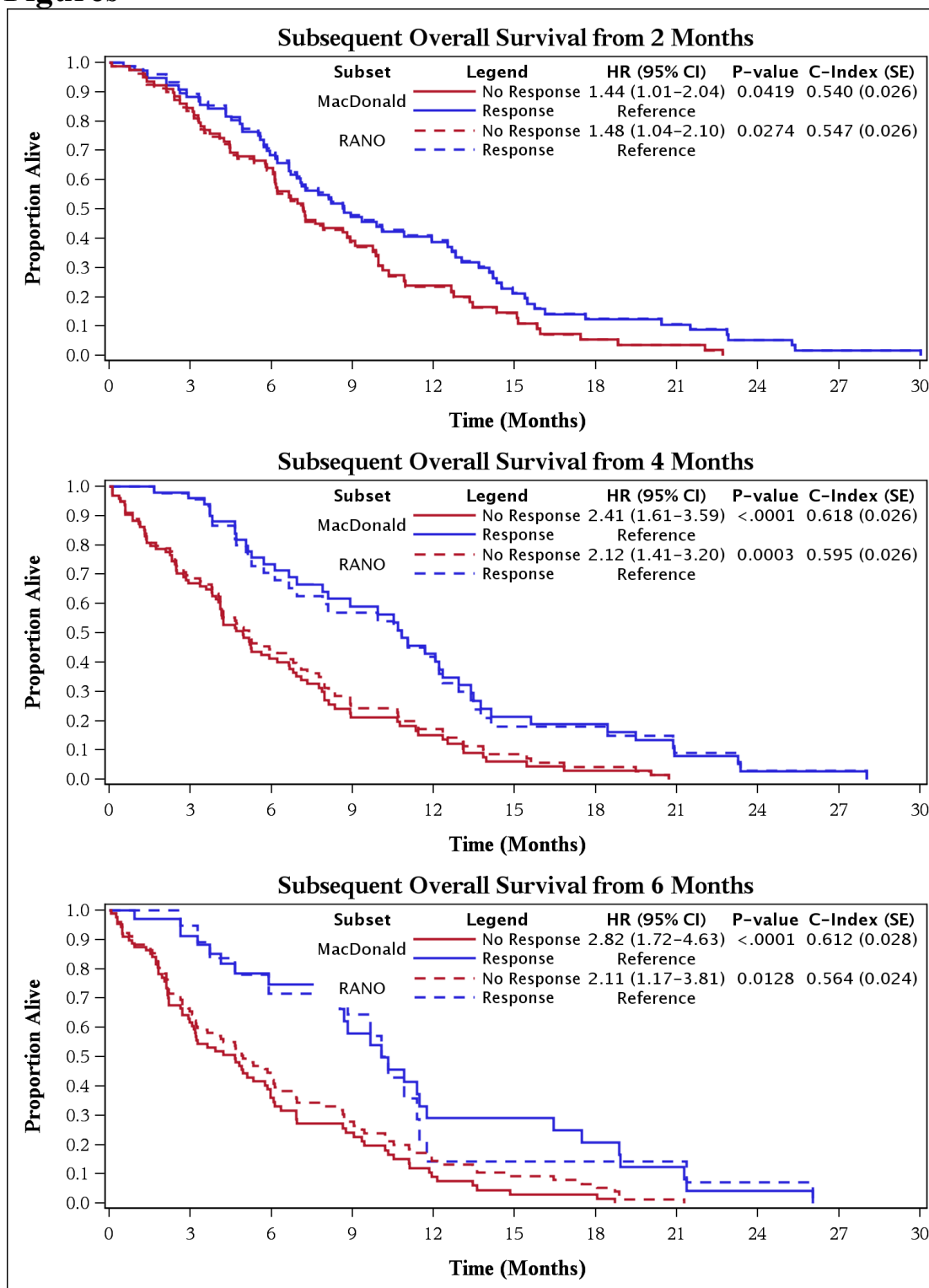
Figure 1: Kaplan-Meier curves of subsequent survival by response in landmark analysis performed at 2, 4 and 6 months.
