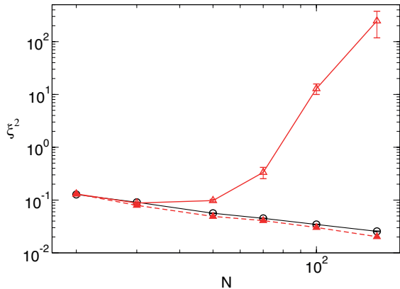
FIG. 3: Final squeezing \xi^2 as a function of the size N , for \nu = 500 for the adiabatic (red triangles) and optimal (black circles) dynamics, subject to random telegraph noise with amplitude K_\alpha = K_\beta = 0.05 (empty symbols) and K_\alpha = K_\beta = 0 (full symbols). Data have been averaged over 24 instances of disorder.
