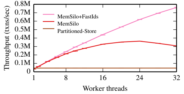
Figure 9: Performance of Partitioned-Store versus MemSilo as the number of workers processing the same size database is varied.
