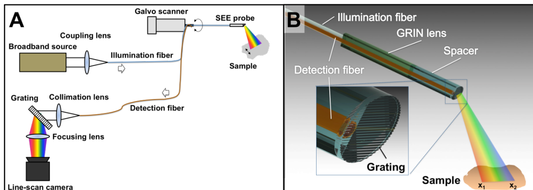
Fig. 1 Schematics of (A) SEE system and (B) SEE probe.
