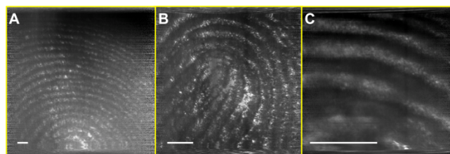
Fig. 3 SEE images of human finger at three different working distances. Scale bar = 1mm.
