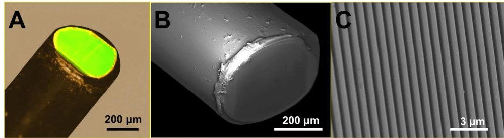
Figure 2 Light microscopy image (A) and SEM images (B and C) of the tip of the SEE probe.
