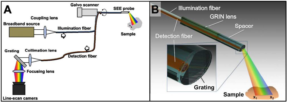
Figure 1 Schematics of (A) SEE system and (B) SEE probe.
