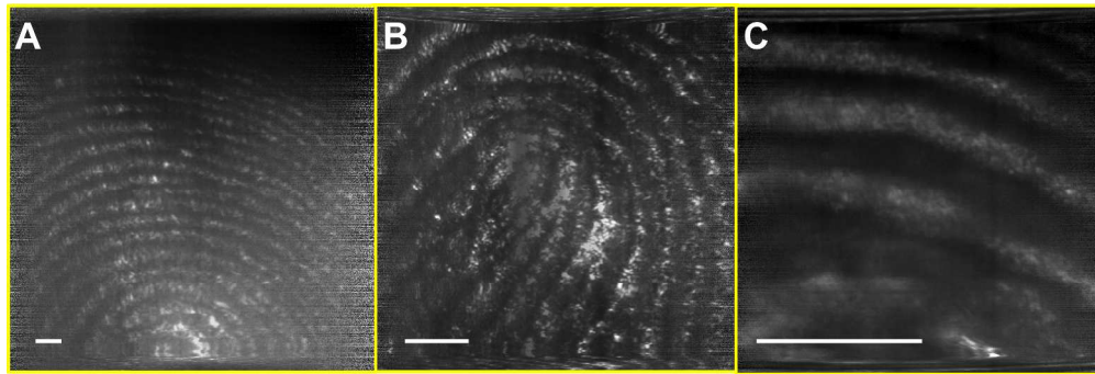
Figure 4 SEE images of human finger at three different working distances. Scale bar = 1mm.
