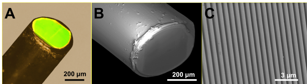
Fig. 2 Light microscopy image (A) and SEM images (B and C) of the tip of the SEE probe.
