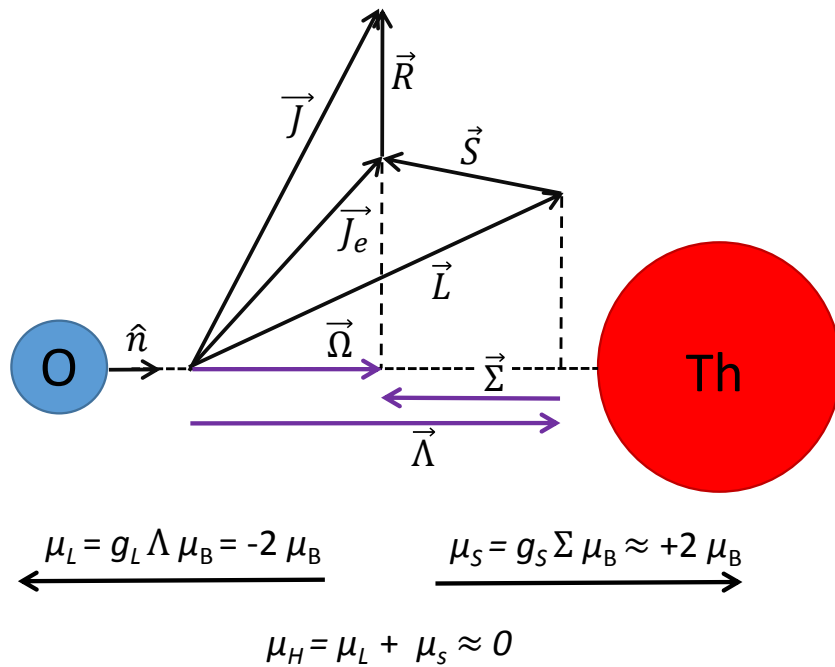
Figure 2.1: The {}^3\Delta_1 (H) state of ThO, with all angular momentum quantum numbers shown. Because projections of the orbital and spin angular momenta on the internuclear axis point in opposite directions, their contributions to the total magnetic moment almost perfectly cancel.
