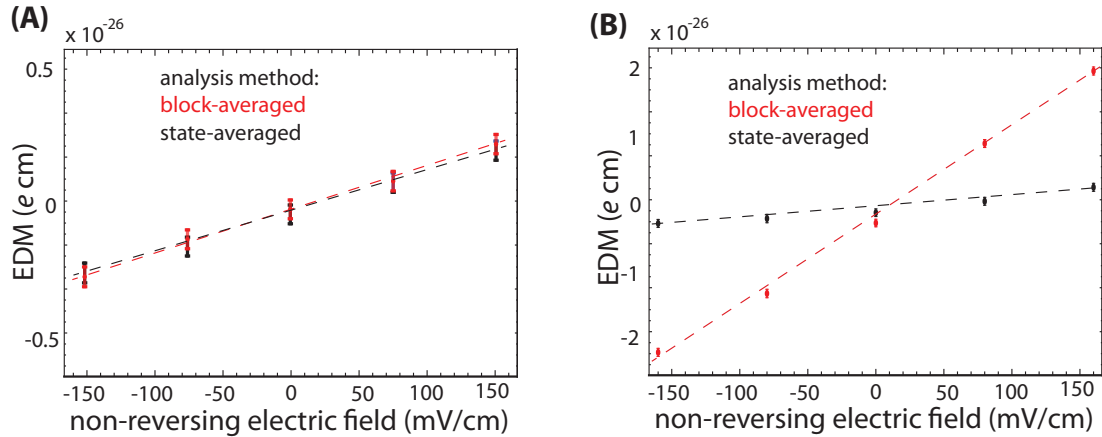
Figure 6.6: (A) Measured EDM vs non-reversing electric field, \mathcal{E}_{NR} , with no correlated contrast. The block- and state-averaged contrast analyses agree for all \mathcal{E}_{NR} values. The small EDM dependence on \mathcal{E}_{NR} is caused by a separate systematic effect discussed in detail in the next chapter. (B) Here there is a significant \tilde{\mathcal{N}}\tilde{\mathcal{E}} -correlated contrast that scales with \mathcal{E}_{NR} . For the block-averaged contrast analysis, this produces a significant EDM systematic shift that also scales with \mathcal{E}_{NR} . However when the EDM is computed with state-averaged contrast, there is no systematic shift from the correlated contrast.
