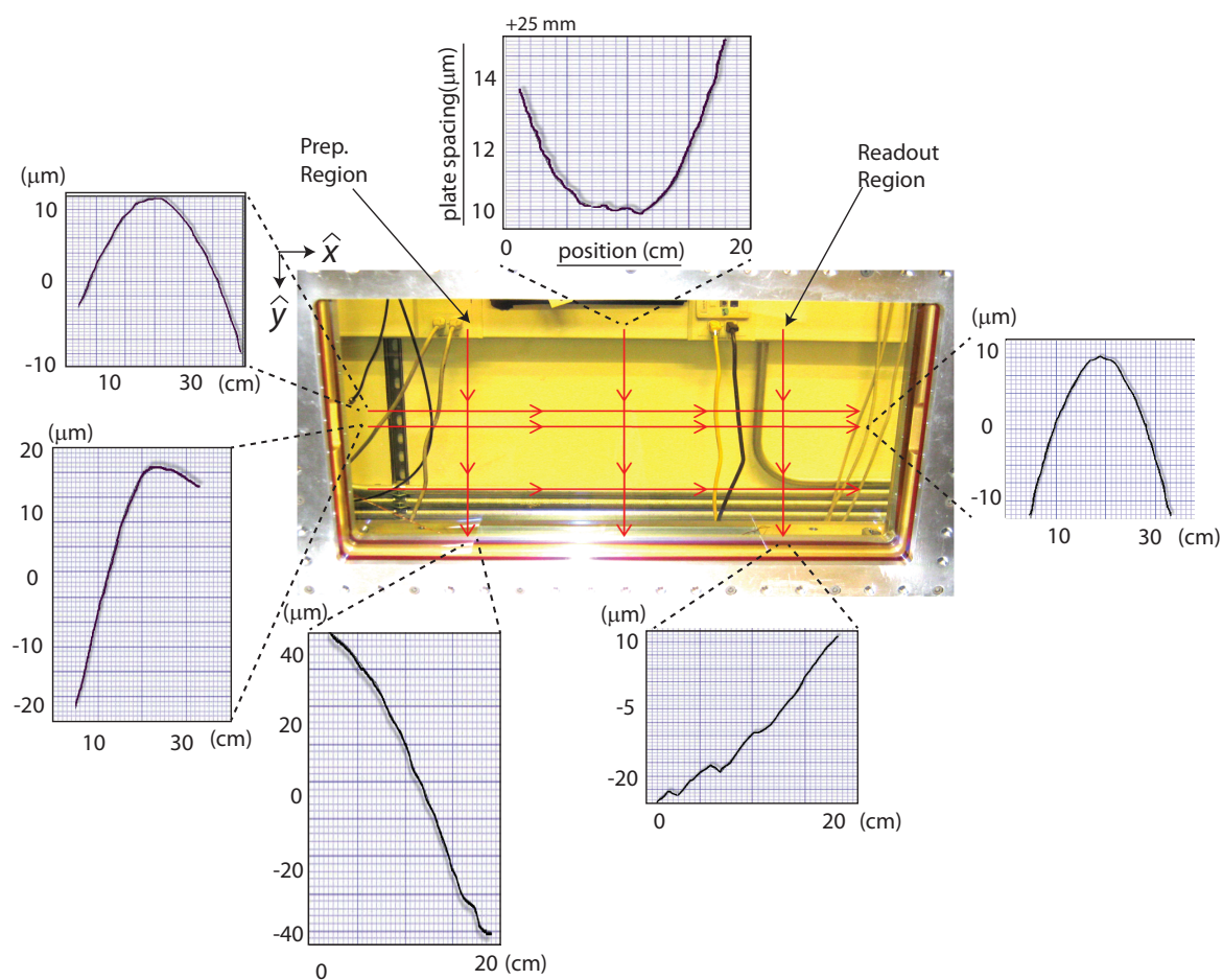
Figure 5.5: Electric field plate spacing, after plate alignment was optimized, measured with a scanning Michelson interferometer along several field plate cross-sections. Multiple scans indicate a saddle-like contortion along the diagonal axis. The plates are positioned to minimize the gradient along the molecule beam line (far right).
