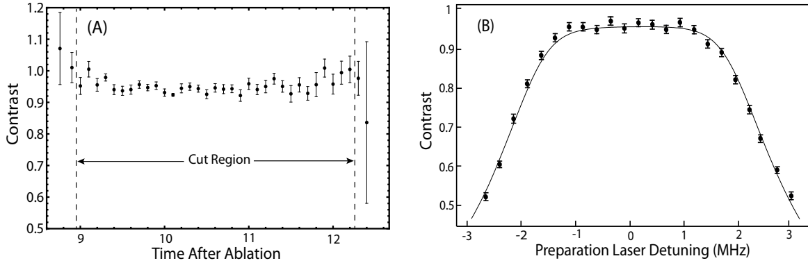
Figure 6.3: Contrast vs time after ablation (A), averaged over 64 traces, and detuning (B), with each point corresponding to 64 averaged traces.
