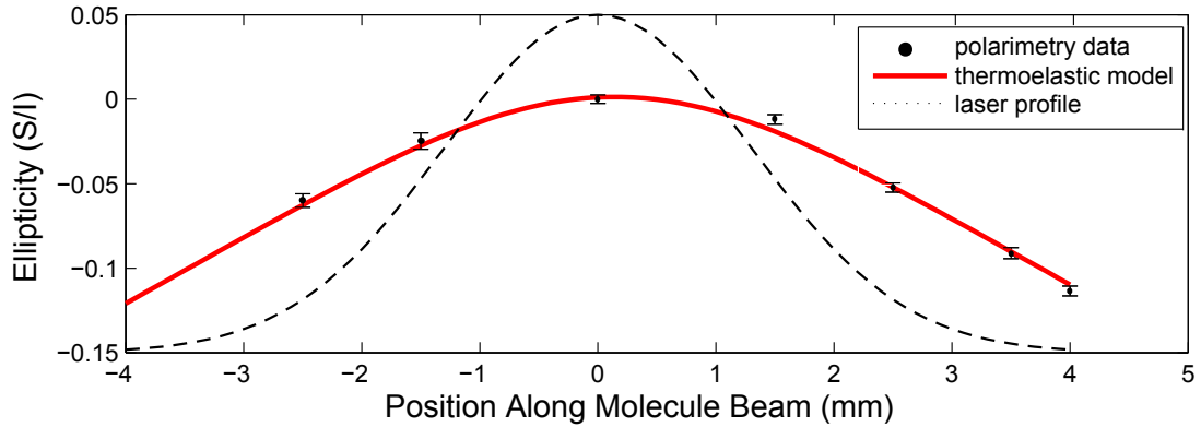
Figure 7.8: Measurements of ellipticity (quantified by Stokes parameters S and I) across the preparation and readout laser beams show a clear circular polarization gradient [71]. This data agrees with a thermoelastic model of the effects of laser-induced heating of the field plates [61]. Polarimetry measurements were performed by Paul Hess and the thermoelastic analysis was performed by Nick Hutzler.
