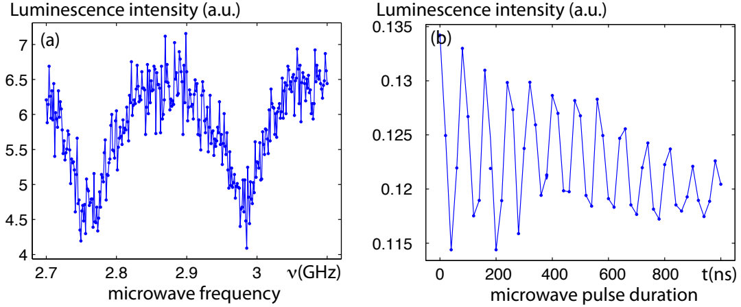
Figure A.5: (a) Spin transition observed in the NV fluorescence under excitation with a microwave field at frequency \nu . (b) Driven spin oscillations for \nu = 2.77 GHz.
