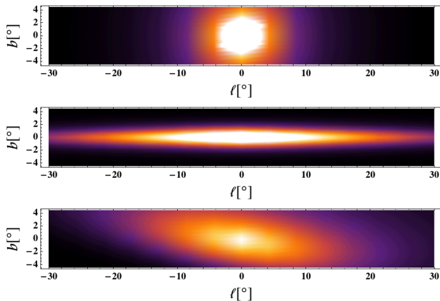
FIG. 3. Sky maps of the photon flux shape, in arbitrary units, for different DM profiles. Upper: Ordinary DM with an Einasto distribution. Middle: DDDM in a disk with scale height z_d = 100 pc, aligned with our disk. Lower: DDDM in a similar disk, now misaligned with our disk by 18^\circ .
