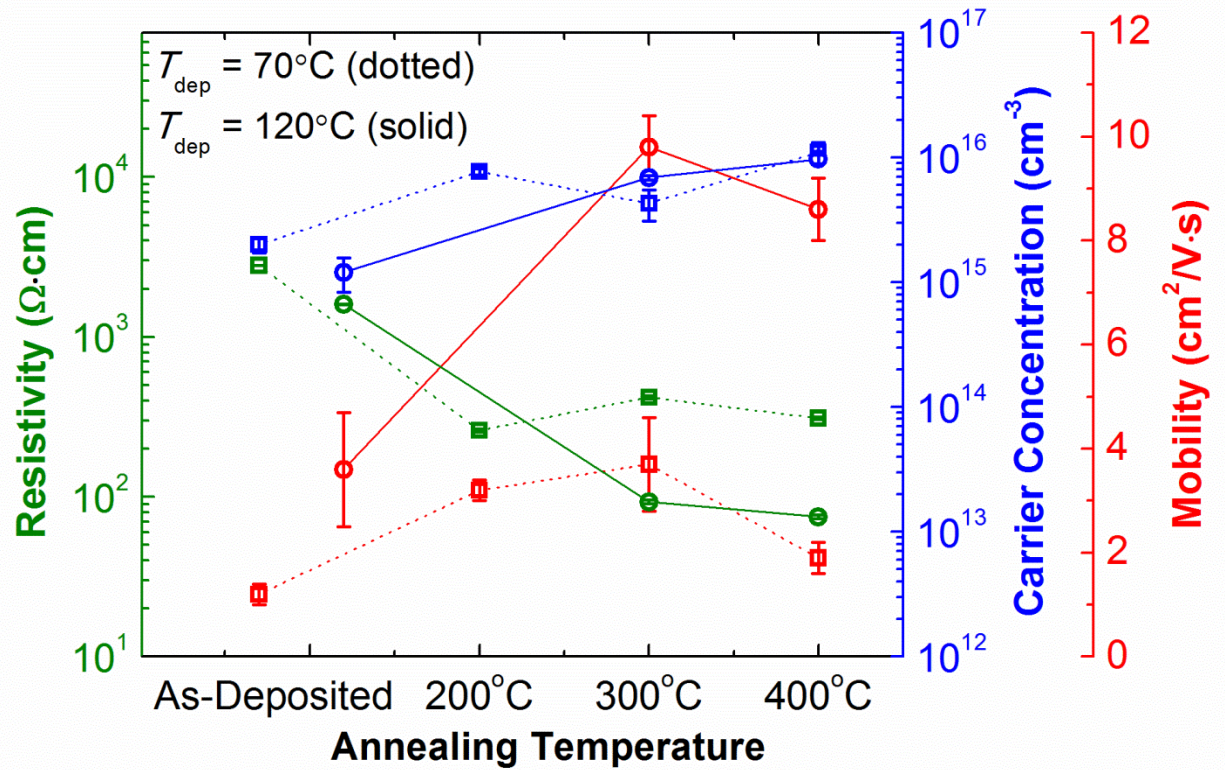
Figure 2. (Color) Plot of resistivity (green), hole carrier concentration (blue), and hole mobility (red) vs. annealing temperature in \text{H}_2\text{S} , for SnS films deposited at 70^\circ\text{C} (dotted) and 120^\circ\text{C} (solid). Resistivity and carrier concentration are plotted on a semilog scale, whereas mobility is plotted on a linear scale.
