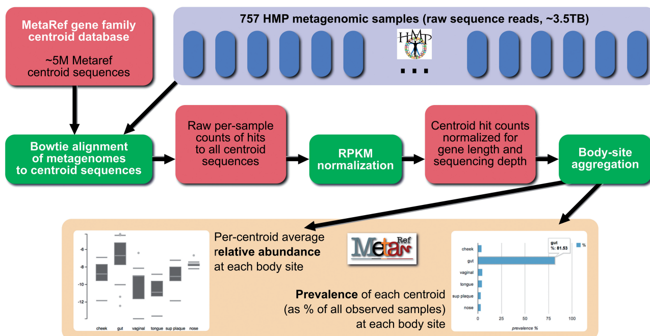
Figure 4. Overview of MetaRef's statistical processing of microbial gene families in the healthy human body-site-specific microbiome. Raw sequence samples from HMP metagenomes are aligned against all MetaRef family centroids; the number of reads aligning to each centroid in each sample is tallied; read counts are transformed via RPKM to normalize with respect to centroid length and sampling depth; centroid RPKMs for all samples associated with each body site are aggregated into measures of prevalence and relative abundance for all centroids detected at that site.
