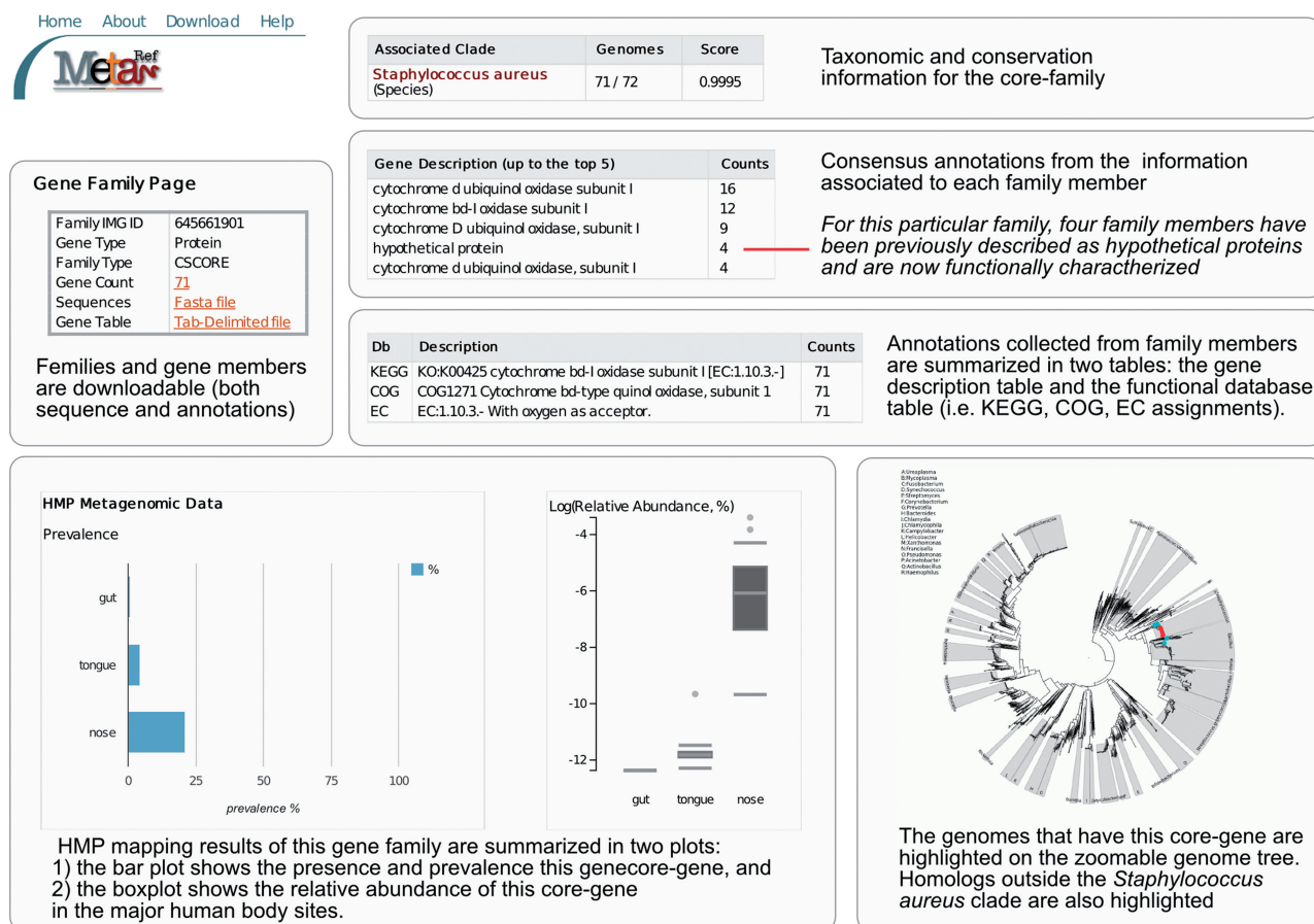
Figure 3. Summary of the main MetaRef panels reported in the family-centric view. For each gene family, MetaRef reports taxonomic, phylogenetic and conservation information as well as available functional information, additional consensus annotations, and the family's prevalence and abundance in human-associated microbiomes. The information can further be analysed interactively (by exploring sub-branches of the microbial phylogeny) and offline (by downloading sequence FASTA files and gene annotation tables for the family).
