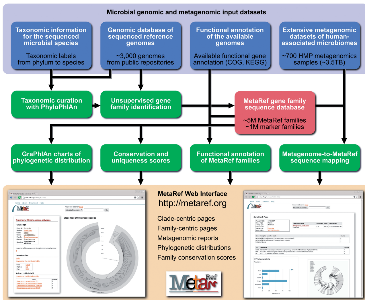
Figure 1. MetaRef comprises automated processing of available microbial genomic information, downloadable phylogenetic and functional annotations, and the MetaRef web portal. The implemented computational pipeline first processes the available microbial reference genomes with the associated taxonomic metadata (currently from IMG) to produce the comprehensive MetaRef sequence database of all gene families. The database is then integrated with the available functional annotations and shotgun metagenomic data (currently from the HMP project) to provide clade-centric and family-centric views of the current microbial diversity.
