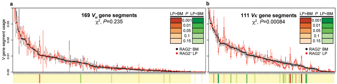
Figure 3. Distinct V segment usage in RAG2^+ cells from BM versus LP a,b , Dot plots show contributions (in order of highest to lowest BM utilization) of different V_{HS} (a) and V_K (b) to in-frame rearrangements in RAG2-GFP^+ BM (black dots) and LP (red dots) cells. The two most highly utilized V_{HS} are omitted to increase plot resolution. Each point shows mean \pm s.e.m. of at least 4 experiments. The \chi^2 calculated P values for overall differences between BM and LP are indicated. Significant V segment utilization differences between BM and LP are indicated on heat map ( P values scale indicated in inset). Full data set at increased resolution is in Supplementary Fig. 12.
