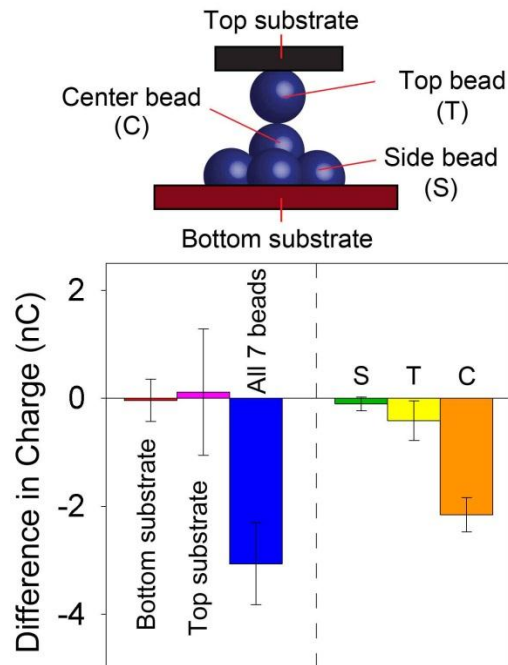
Figure 5. Charge did not dissipate into the solid substrates during contact de-electrification. The charges of the already-charged Nylon beads and the substrates were measured before and after contact de-electrification. Charges on the top and bottom substrates did not change significantly compared to the overall reduction in the charge of all the seven beads involved; this result shows that charges did not transfer from the beads into the substrate. The differences in charge on each side, top and center bead are also shown in this plot. ( n = 7 )
