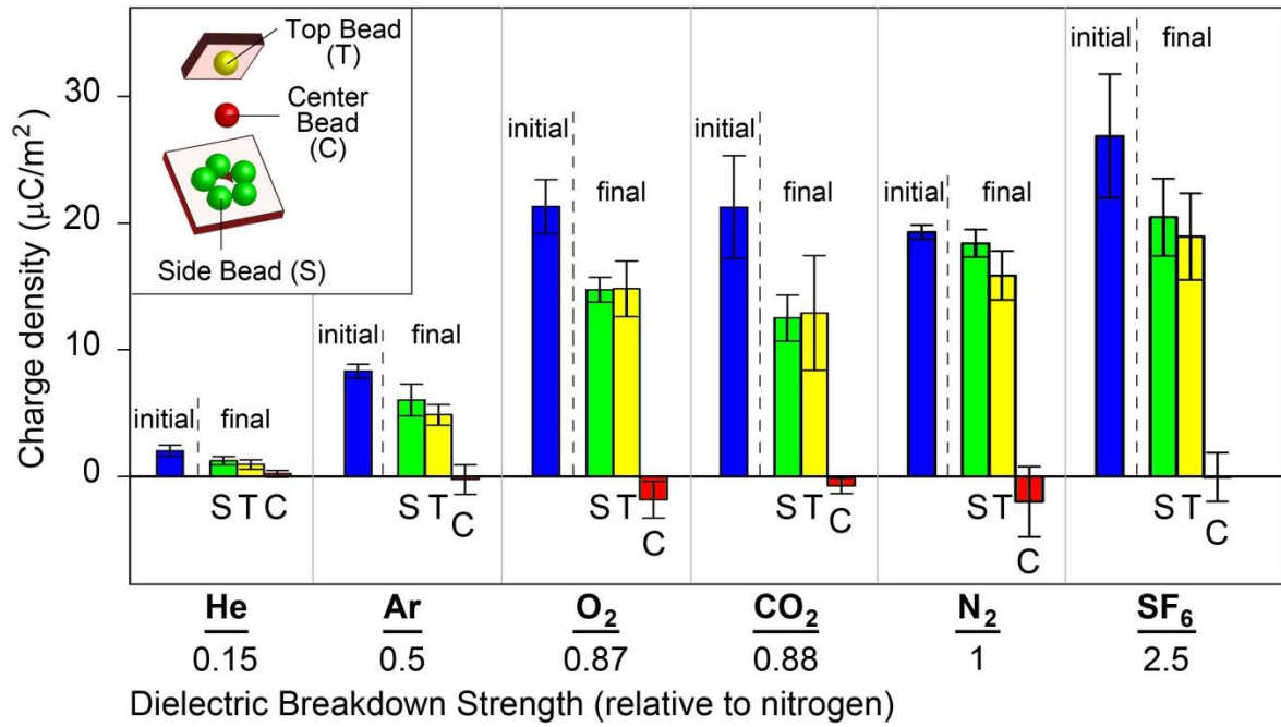
Figure 4. Contact de-energization occurred under different types of gaseous atmosphere. Despite different amounts of initial charge on the Nylon beads under different atmospheres, the center bead discharged almost completely after being brought into contact with the top bead for all cases. ( n \geq 7 )
