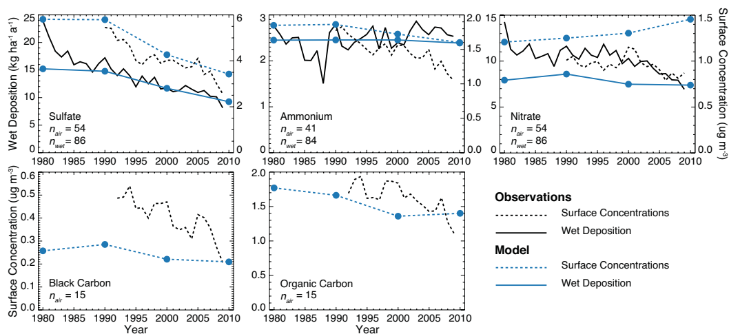
Fig. 3. 1980–2010 trends in wet deposition fluxes (solid) and surface aerosol concentrations (dashed) in the eastern US (east of 100^\circ W). Values are annual means. Model trends (blue) are compared to observations (black). The number of sites averaged in each calculated trend is given inset. Model values are sampled at the site locations and then averaged.
