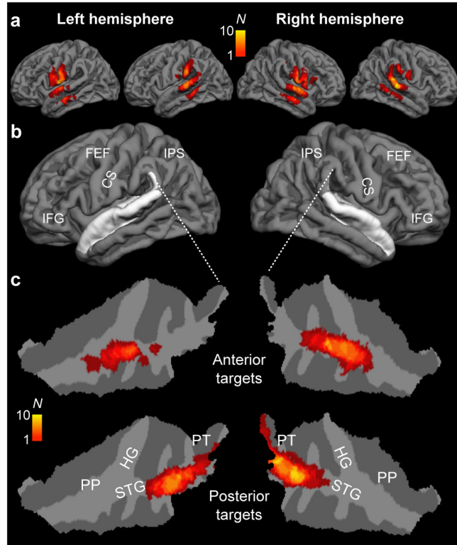
Figure 4. Modeling of TMS-induced E-fields in the cortex. (a) Distribution of TMS effects exceeding 80% motor threshold (MT) strength during TMS in all subjects ( N=10 ), shown on a standard brain cortical reconstruction. (b) Gross anatomical landmarks of interest shown on the standard-brain cortex. The location of superior temporal cortices, which encompass ACs has been shown in white. The loci of central sulcus (CS), and extra-AC areas related to “what” (inferior frontal gyrus, IFG) and “where” (intraparietal sulcus, IPS; frontal eye fields, FEF) processing streams are also shown. (c) TMS-induced electric fields in AC on flattened patches of the superior temporal cortices. Taken together, our modeling results demonstrate that TMS-induced E-fields were successfully delivered at the posterior (posterior STG, PT) vs. anterior AC areas (anterior STG, PP), hypothesized to be associated with sound location vs. identity feature discrimination, respectively. As expected, TMS also induced E-fields in the adjacent cortical gyri. However, the panel a shows that these fields were not close to the frontoparietal areas typically associated with extra-AC “where” (IPS/FEF) and “what” (IFG) processing. The color scale depicts the number of subjects with stimulation reaching the threshold at a given location.
