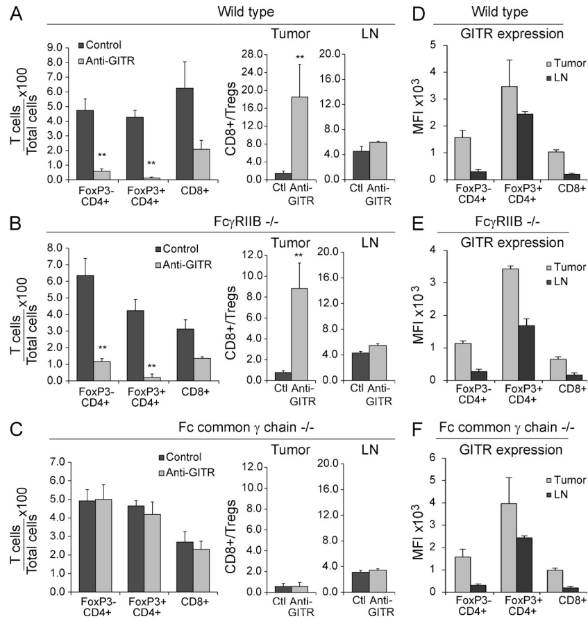
Figure 4. Activating, but not inhibitory, Fc \gamma R are required for intratumoral T reg cell depletion by antibodies targeting GTR. Intratumoral T cell density and CD8 + T cells to T reg cells ratios 5 d after treatment with 5 mg/kg DTA-1-mIgG2a using wild-type (A), Fc \gamma RIIB -/- (B), or Fc common \gamma chain -/- (C) mice bearing Colon26 tumors. (D–F) Cell surface expression of GTR on T cells. Mean and standard errors are based on triplicates from two independent experiments. P-values were calculated using an unpaired Student’s t test (**, P < 0.001).
