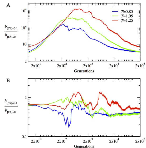
Figure 2. The time evolution of the fitness ratios b_{[Ch]=0.1}/b_{[Ch]=0} (i.e. the ratio of birth rates with chaperones and without chaperones) are presented for the active x = 0.1 in (A) and passive x = 0 model in (B) for three different temperatures. The fitness ratios and evolutionary time are in log scale to convey the events clearly across all time scales. All data here and in the subsequent figures are ensemble averages over 100 independent stochastic trajectories. doi:10.1371/journal.pcbi.1003269.g002
