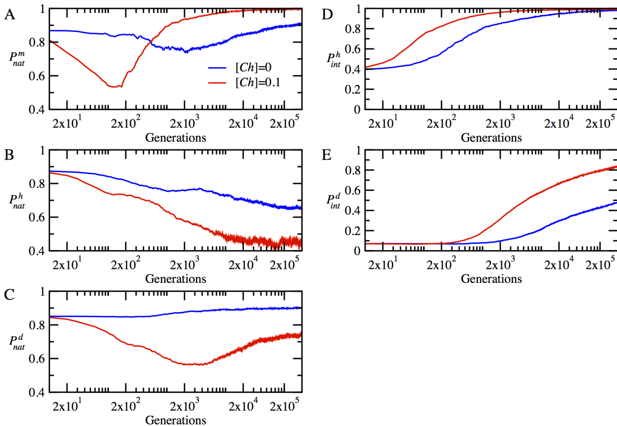
Figure 3. The time evolution of mean protein stabilities and mean interaction probabilities of functional dimers in the absence and presence of chaperones, i.e. for [Ch]=0 (blue lines) and [Ch]=0.1 (red lines), respectively, at temperature T=0.85 . (A) The time evolution of stability P_{nat}^m = P_{nat}^1 for monomeric proteins. (B) The time evolution of mean stability, P_{nat}^h = (P_{nat}^2 + P_{nat}^3)/2 for heterodimer proteins. (C) The time evolution of mean stability, P_{nat}^d = (P_{nat}^4 + P_{nat}^5 + P_{nat}^6)/3 for date triangle proteins. (D) The time evolution of interaction probability, P_{int}^h = P_{int}^{23} for the heterodimer complexes. (E) The time evolution of mean interaction probability, P_{int}^d = (P_{int}^{45} + P_{int}^{46} + P_{int}^{56})/3 for the date triangle complexes.
