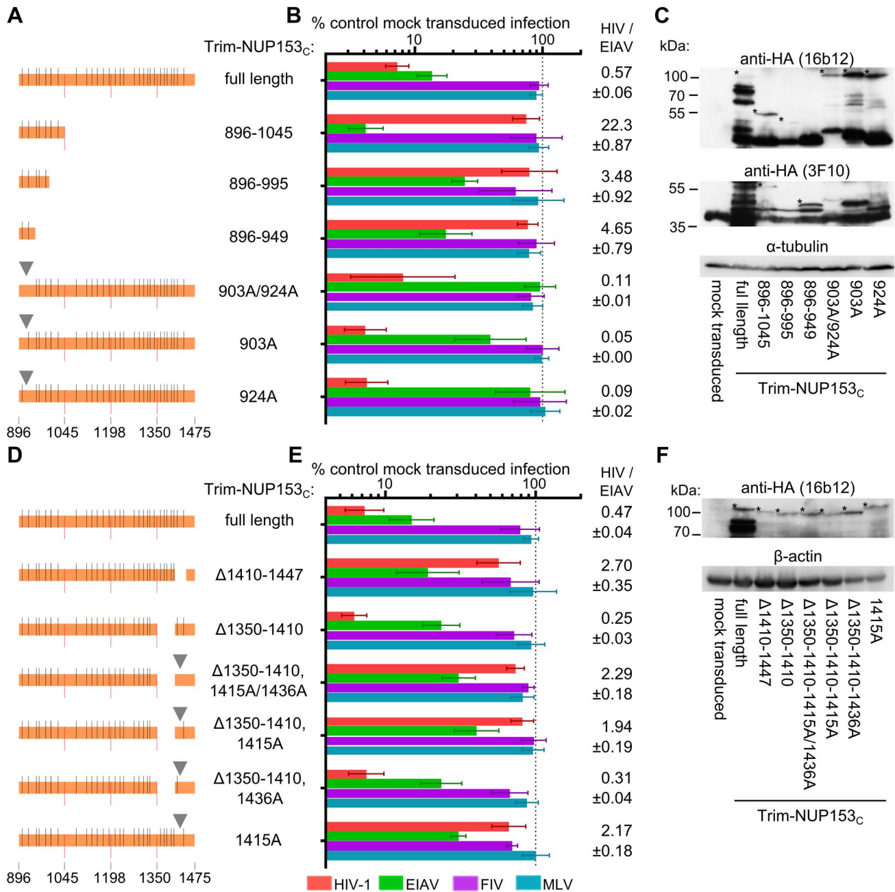
Figure 5. The importance of FG motifs for Trim-NUP153 C mediated inhibition of HIV-1 and EIAV infection. To-scale schematics (A and D), normalized infection data (B and E), and western blotting (C and F) as described for Figure 4. Infection data are the geometric mean of at least 4 experiments, with error bars denoting 95% confidence intervals. Inverted grey triangle (panels A and D) denotes area of missense mutation. doi:10.1371/journal.ppat.1003693.g005
