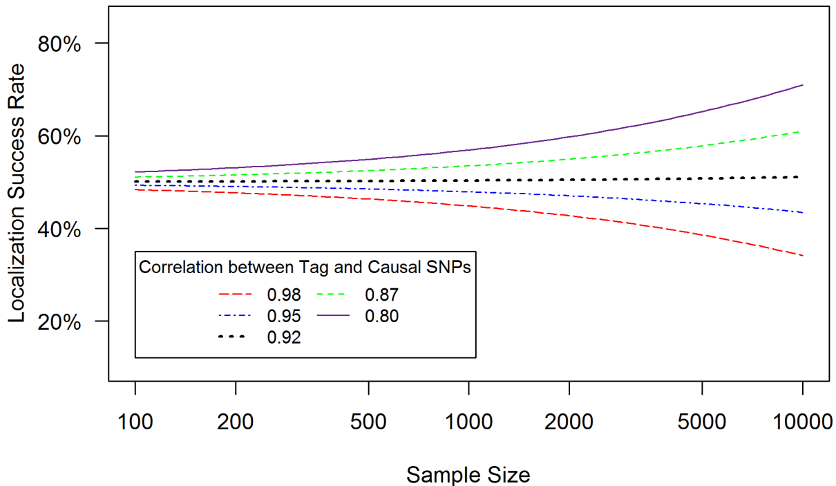
Figure 3. Well-tagged causal SNPs sequenced with low accuracy are unlikely to be correctly identified even as sample size increases. Localization success rates for association studies (sample size from 50:50 cases:controls to 5000:5000 cases:controls, X-axis) of one causal SNP (MAF = 0.12; OR = 1.25; imperfect genotyping accuracy due to sequencing or imputation errors resulting in correlation between the actual and estimated genotypes \rho_C = 0.95 ) and one tag SNP (MAF = 0.12; in high correlation with the causal SNP, r_{CG} = 0.8 (purple solid) to 0.98 (red dashed); 100% genotyping accuracy with \rho_G = 1 ) with no selection for significance at the tag SNP. doi:10.1371/journal.pgen.1003609.g003
