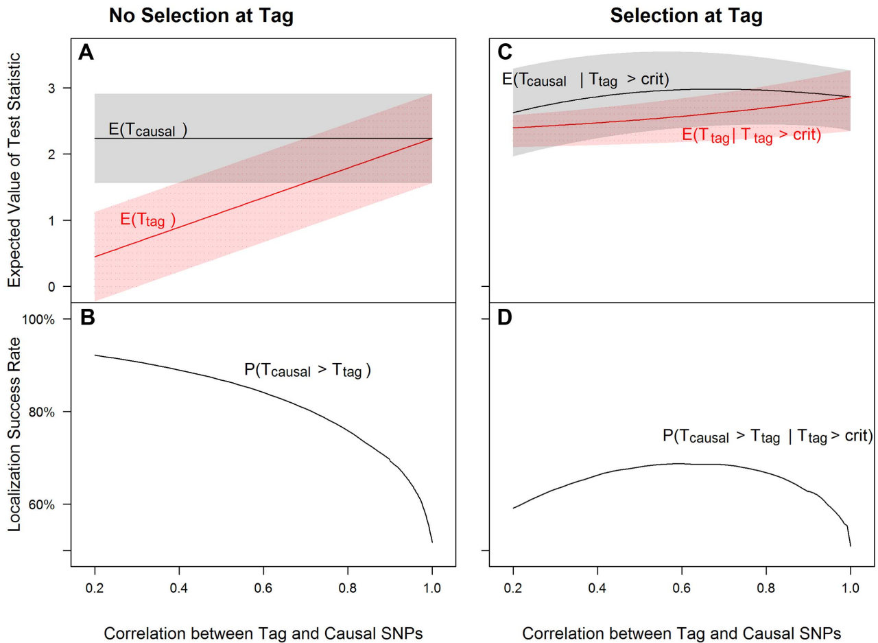
Figure 1. Tagging effect decreases localization success rates with or without the selection effect. The expected values of the association test statistics at a tag SNP (red) and the causal SNP (black), shading from 25 th –75 th percentiles ( A , C ), and the localization success rates ( B , D ) for association studies (1000 cases and 1000 controls) of one causal SNP (MAF = 0.12; OR = 1.25; perfect genotyping accuracy) and one tag SNP (MAF = 0.12; in varying degree of correlation with the causal SNP, r = 0.2 to 1; perfect genotyping accuracy) with no selection for significance at the tag SNP ( A , B ) or selection at the tag SNP requiring the test statistic T_G to be significant with p\text{-value} < 0.05 ( C , D ). doi:10.1371/journal.pgen.1003609.g001
