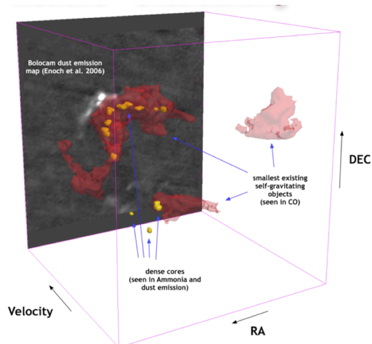
Fig. 8 “Astronomical Medicine” view of L1448, created using 3D Slicer by Jens Kauffmann. Similar figures were published as the first interactive 3D PDFs in the journal Nature (Goodman et al. 2009).
