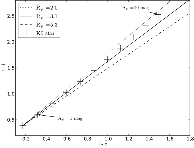
Figure 6. Red-optical ( r - i versus i - z ) colours of a Castelli & Kurucz (2004) model K0V star produced in SYNPHOT by convolving the stellar spectrum with the filter response curves for the MMT. The stellar spectrum is reddened with a CCM R_V = 3.1 reddening law in steps of A_V = 1 magnitude (plus symbols). The change in the effective wavelength of the reddened spectrum causes the colours to trace out a curved line in colour-colour space, rather than the straight vectors assumed in our model (straight lines). This effect makes it look as if a star behind more extinction is being reddened by an extinction law with a smaller R_V .
