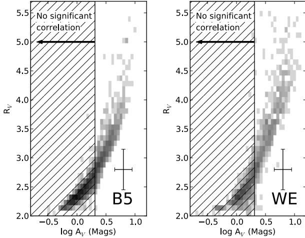
Figure 9. The mean and standard deviations of the marginal posterior distributions of A_V and R_V for all the stars in our data samples for B5 (left panel) and the West-End (right panel) from our hierarchical Bayesian model. The shade of grey shows the density of points at a position within the diagram. A representative error bar is shown, which displays the median width of the posterior probability distribution for A_V and R_V for a single star (rather than for one of the bins displayed in this figure). Note that the widths of the posterior probability distributions for A_V and R_V vary greatly among individual stars. When we include only sources with A_V < 2 magnitudes the correlation between A_V and R_V is no longer distinguishable from zero. For these points we are unable to infer any underlying correlation and the tight relationship seen in this diagram is due to the strong correlation inferred for stars with A_V > 2 magnitudes.
