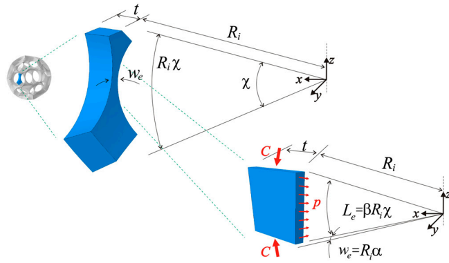
Fig. S3. Representative ligament extracted from the Buckliball and simplified curved column used in its buckling analysis.
