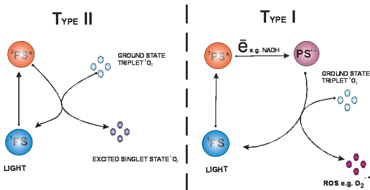
Figure 3. Photodynamic effect. An excited triplet state can either react directly with a reductant, e.g., an organic molecule in a cellular microenvironment, acquiring a hydrogen atom or electron to form a radical and produce a superoxide anion radical (O 2 •- ), type I reaction or, more likely, transfer its energy to molecular oxygen ( 3 O 2 ) and form singlet oxygen ( 1 O 2 ), type II reaction.
