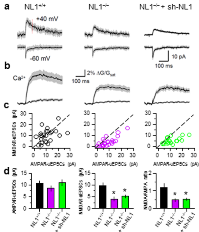
Figure 3. Constitutive NL1 knock-out lowers NMDAR-uEPSCs and Ca 2+ transients (a and b) Average AMPAR- and NMDAR-uEPSCs (a) and spine and dendrite Ca 2+ transients at -60 mV (b) for neurons of the indicated genotypes. (c) Relationship between AMPAR- and NMDAR-uEPSCs measured in the indicated genotypes. (d) Average amplitudes of AMPAR- ( left ) and NMDAR- ( middle ) uEPSCs and NMDAR/AMPA current ratios ( right ).
