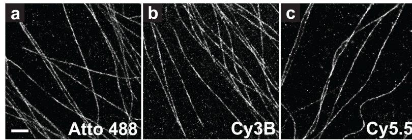
Figure 2. STORM images of microtubules in cells stained by indirect immunofluorescence with (a) Atto 488, (b) Cy3B, and (c) Cy5.5. Samples were reduced in situ with \text{NaBH}_4 , washed, and then imaged with 488 nm, 561 nm, and 647 nm excitation light in a buffer designed to reduce blinking and photobleaching. Illumination with 405 nm light allowed control over the activation rate. Scale bar, 1 \mu\text{m} .
