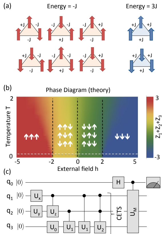
FIG. 1: Theoretical descriptions of the frustrated magnet. (a) All possible configurations of a three-spin frustrated magnet at zero temperature and zero magnetic field. There is a six-fold degeneracy in the ground state, leading to a non-zero entropy. (b) Theoretical phase diagram. The units of the axes are k_B and J for temperature and external field. The dashed line parallel h -axis denotes T = 1/11 , which corresponds to the case of the experimental data taken in fig. 3. (c) Quantum circuit diagram for preparing and measuring the CETS |\Psi_\beta\rangle defined in Eq. 1 from the initial state |0000\rangle . The gate sequence for preparing the CETS on the lower three qubits is determined by the method in Ref. [18]. An explicit way for constructing the U_k -gates is given in the supplementary materials. The top qubit q_0 serves as a probe for measuring the physical observables.
