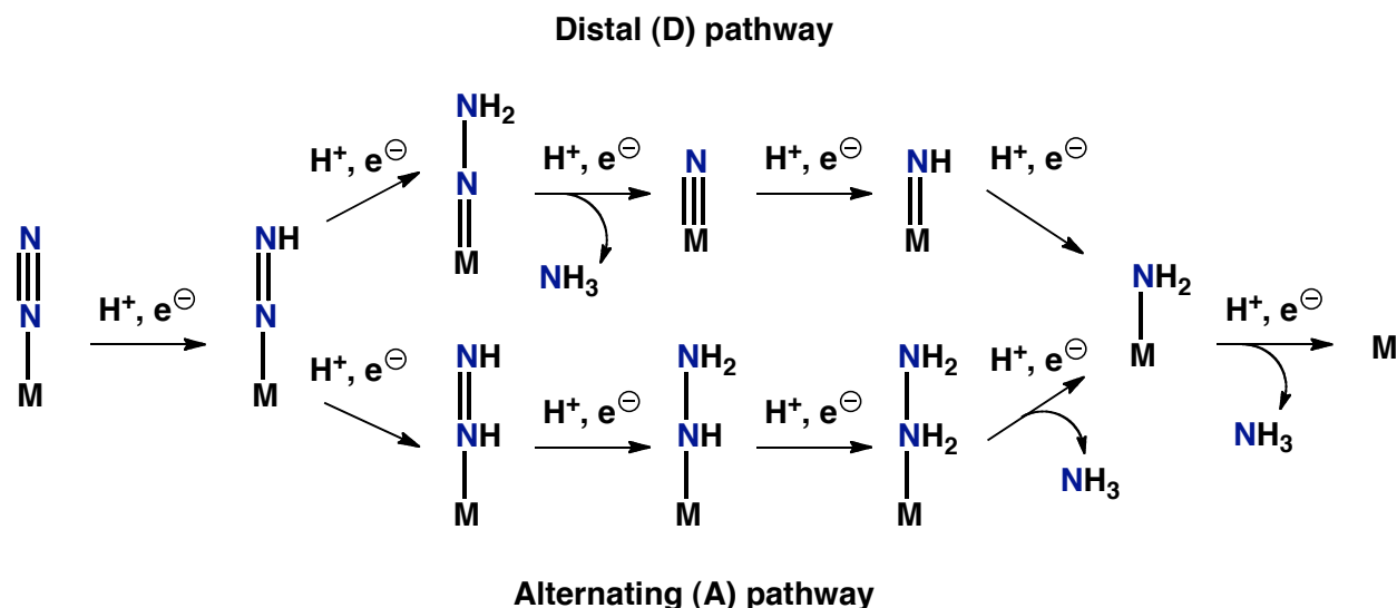
Figure 1.6. Two proposed mechanistic pathways for N 2 reduction by nitrogenase: distal (D) pathway and alternating (A) pathway.
