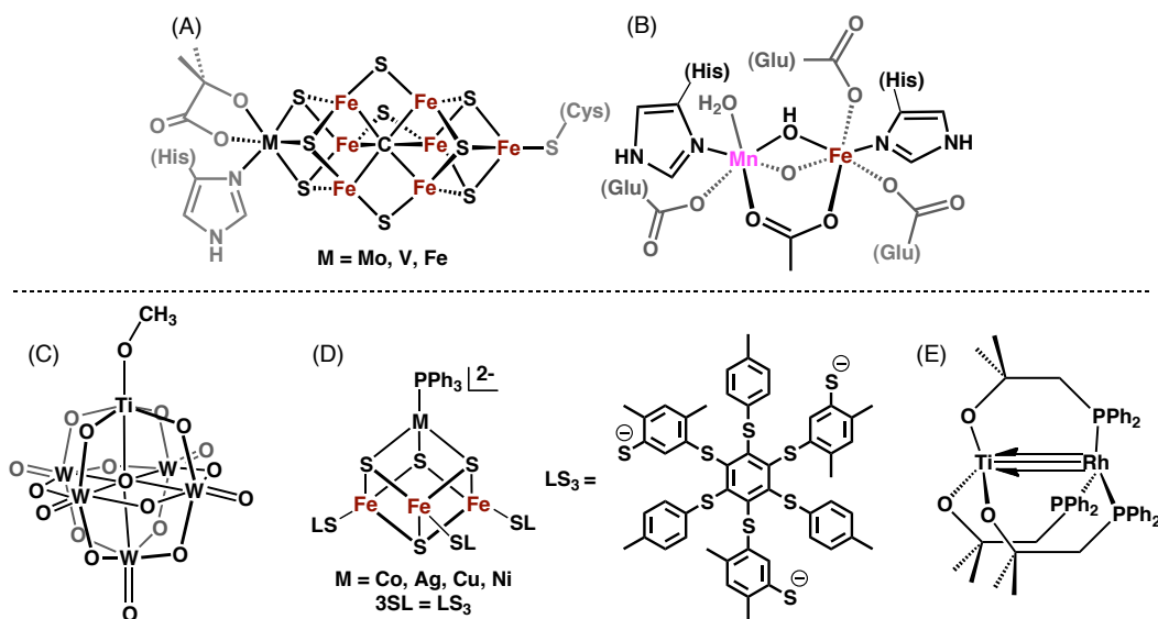
Figure 5.1. Examples of metalloenzymes featuring bimetallic cofactors: (A) FeMoco of nitrogenase and (B) proposed Fe(III)Mn(IV) cofactor of ribonucleotide reductase (note: site-placement of metal ions unknown). 233 Examples of previously synthesized bimetallic compounds accessed by (C) self-assembly methods (e.g. polyoxometalates), 235,236 (D) reaction of incomplete clusters (e.g. cuboidal \text{Fe}_3\text{S}_4 clusters) 3,237,238 with divalent transition metal or alkaline ions, and (E) polynucleating ligands that have different elemental binding affinities (heterobimetallic Ti/Rh cluster). 239
