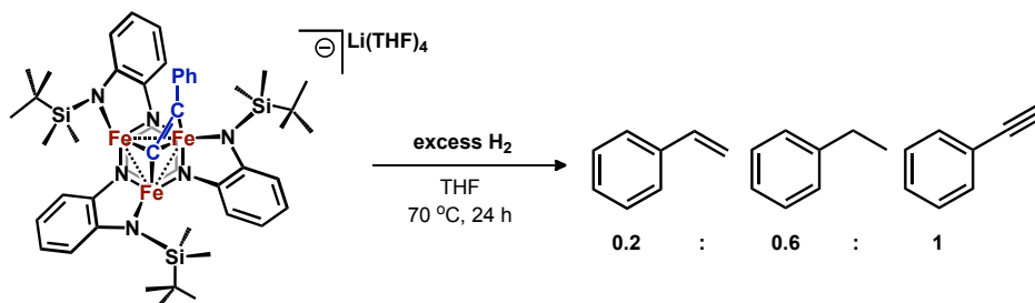
Scheme 4.3. Hydrogenation of acetylide moiety in (^{\text{tbs}}\text{L})\text{Fe}_3(\mu^3\text{-}\eta^2\text{-CCPh})^-
