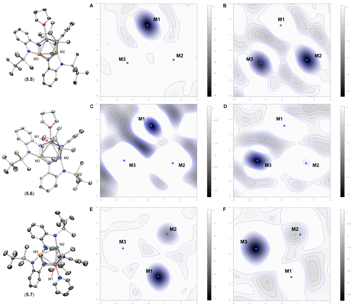
Figure 5.7. Anomalous difference Fourier maps at the Mn and Fe absorption edges of compounds (^{tbs}\text{L})\text{Fe}_2\text{Mn}(\text{THF}) ( 5.5 ) (A and B), (^{tbs}\text{L})\text{Mn}_2\text{Fe}(\text{THF}) ( 5.6 ) (C and D), and (^{tbs}\text{L})\text{Mn}_2\text{Fe}(\text{pyr}) ( 5.7 ) (E and F). Maps A, C, and E were calculated with dataset 3 (at the Mn absorption edge) and maps B, D, and F were calculated with dataset 6 (at the Fe absorption edge).
