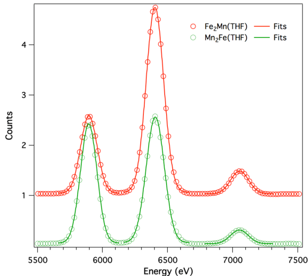
Figure 5.6. X-ray fluorescence spectra of Fe 2 Mn(THF) complex 5.5 (red trace) and Mn 2 Fe(THF) complex 5.6 (green trace).
