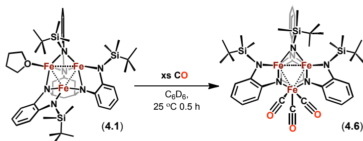
Scheme 4.4. Synthesis of (^{tbs}L)Fe_3(\mu^1-CO)_3
