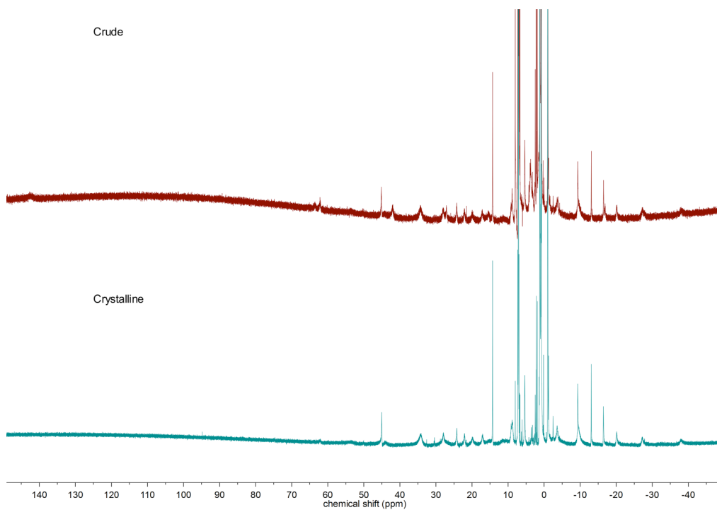
Figure 3.8. 1 H NMR of ( t bsL)Fe 3 (μ 3 -NPh)(μ 2 -NPh) ( 3.5 ) crude and crystalline material.
