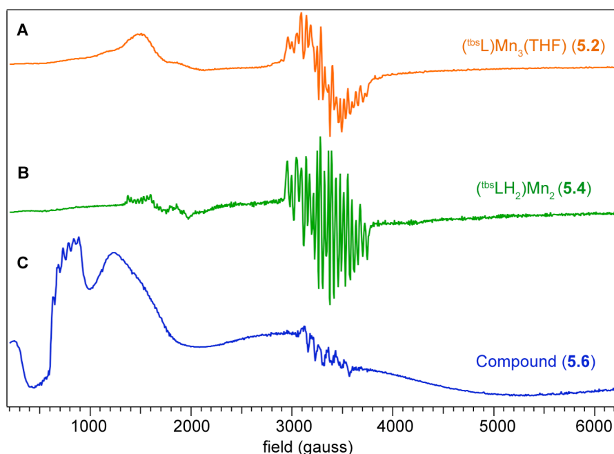
Figure 5.4. EPR spectra of (A) (^{tbs}L)Mn_3(THF) ( 5.2 ) (orange), (B) (^{tbs}LH_2)Mn_2 ( 5.4 ) (green), and (C) crystalline bimetallic trinuclear compound ( 5.6 ) (blue) at 4 K.
