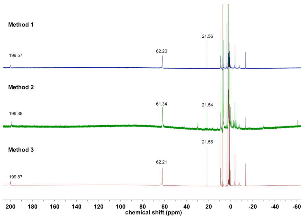
Figure 3.7. ^1\text{H} NMR overlays of methods 1, 2, and 3 to synthesize (^{\text{tbs}}\text{L})\text{Fe}_3(\mu^3\text{-NPh}) ( 3.4 ). Method 1: 3.1 + PhHNNHPh; Method 2: 3.1 + PhNNPh; Method 3: 3.1 + N _3 Ph.
