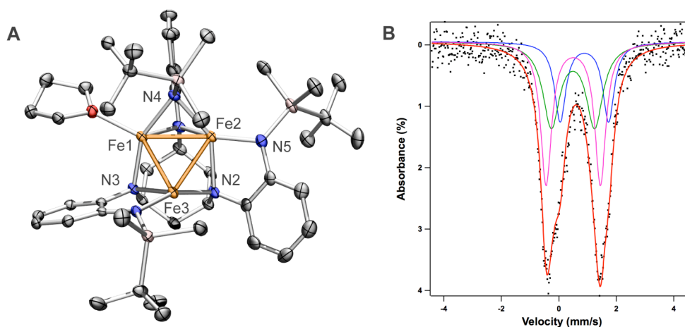
Figure 2.3. (A) Solid-state structure for ({}^{\text{tbs}}\text{L})\text{Fe}_3(\text{THF}) ( 2.8 ) with the thermal ellipsoids set at the 50% probability level (hydrogen atoms and solvent molecules omitted for clarity; Fe orange, C black, H white, N blue, O red, Si pink). Bond lengths (Å): Fe1–Fe2, 2.6129(5); Fe1–Fe3, 2.5061(5); Fe2–Fe3, 2.6118(5); Fe–N int , (N int = N1, N2, N3), 2.047(2); Fe–N Si , (N Si = N4, N5, N6) 1.950(2); Fe–O, 2.1162(18). (B) Zero-field {}^{57}\text{Fe} Mössbauer spectrum of ({}^{\text{tbs}}\text{L})\text{Fe}_3(\text{THF}) obtained at 110 K. Fitting parameters: \delta , |\Delta E_Q| ( \text{mm/s} ) component 1 (blue, 24%): 0.89, 1.69 ( \Gamma = 0.24 \text{ mm/s} ); component 2 (green, 35%): 0.49, 1.51 ( \Gamma = 0.35 \text{ mm/s} ); component 3 (pink, 41%): 0.50, 1.89 ( \Gamma = 0.23 \text{ mm/s} ).
