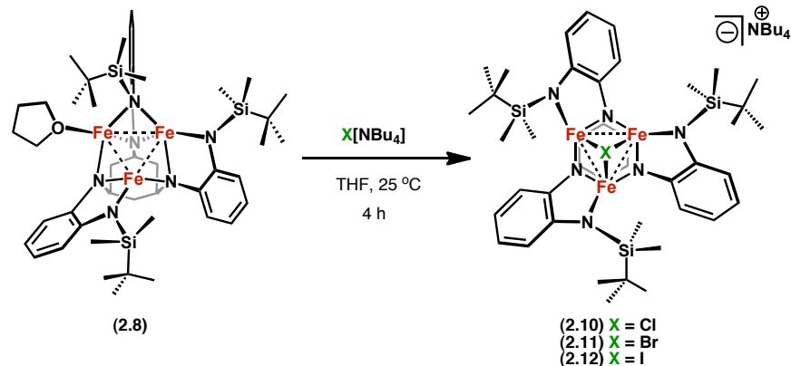
Scheme 2.4. Synthesis of [(^{\text{tbs}}\text{L})\text{Fe}_3(\mu^3\text{-X})]^- , where X = Cl, Br, or I.
