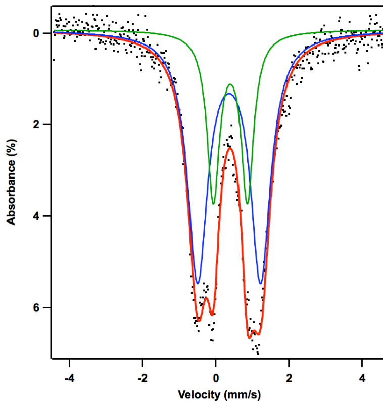
Figure 3.12. Crude zero-field Mössbauer spectrum of (^{55}\text{L})\text{Fe}_3(\mu^3\text{-NPh}) ( 3.4 ) obtained at 90 K prepared by method 2. Fitting parameters: \delta , |AE_Q| ( \text{mm/s} ) component 1 (blue, 69%) 0.37, 1.72 ( \Gamma = 0.33 \text{ mm/s} ); component 2 (green, 31%) 0.41, 0.93 ( \Gamma = 0.21 \text{ mm/s} ).
