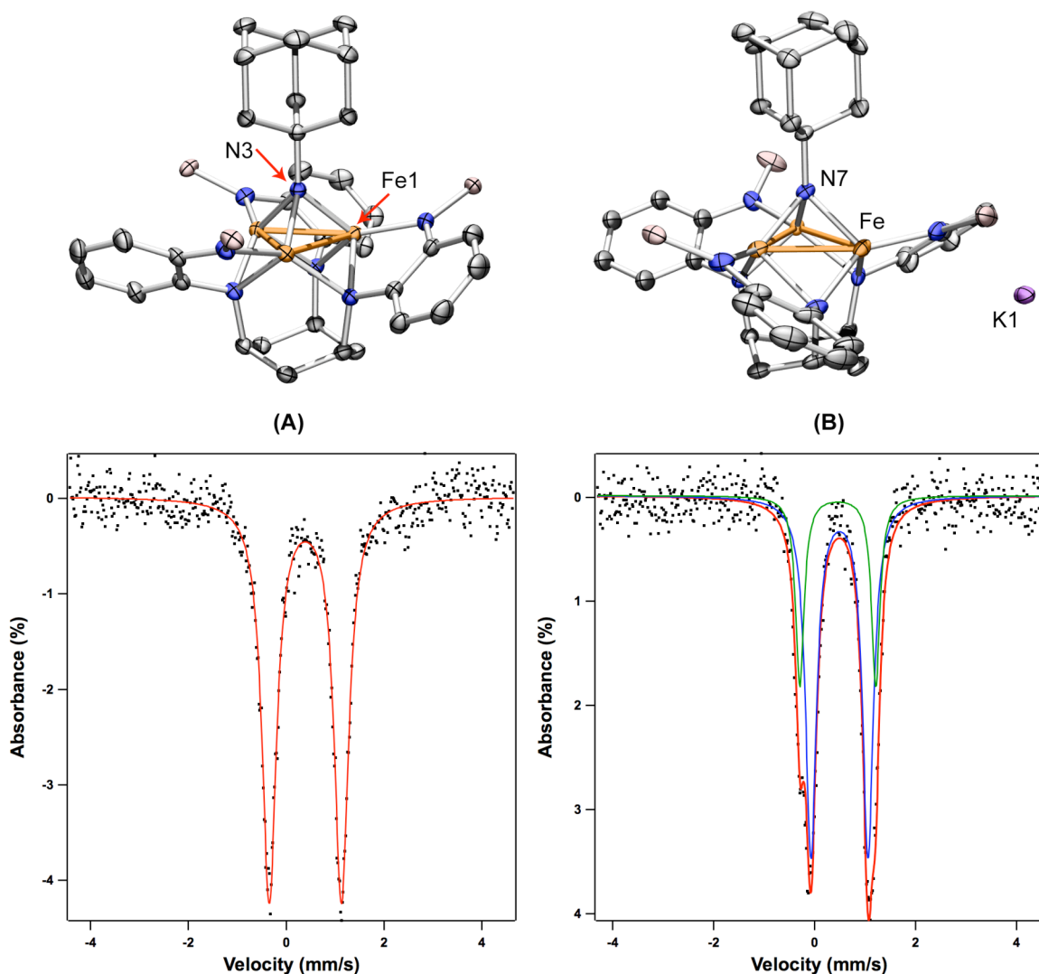
Figure 3.4. Solid-state structures of (A) (^{tbs}L)Fe_3(\mu^3\text{-NAd}) ( 3.7 ) and (B) [(^{tbs}L)Fe_3(\mu^3\text{-NAd})]K(THF)_4 ( 3.8 ) with the thermal ellipsoids set at the 50% probability level (hydrogen atoms, solvent molecules, and alkyl groups on Si omitted for clarity; Fe orange, C gray, N blue, Si Pink, K orchid). Selected bond lengths ( \text{\AA} ) for 3.7 : Fe–Fe, 2.5297(8); Fe–N3, 1.934(3); for 3.8 : Fe– Fe_{\text{avg}} , 2.561(1); Fe– N7_{\text{avg}} , 1.955(4). Zero-field Mössbauer spectrum of (A) ( 3.7 ) obtained at 110 K and (B) [(^{tbs}L)Fe_3(\mu^3\text{-NAd})]K(C_{12}H_{24}O_6) obtained at 105 K. Fitting parameters: (A) \delta ( \text{mm/s} ), |AE_Q| ( \text{mm/s} ) 0.39, 1.48 ( \Gamma = 0.18 \text{mm/s} ) and (B) component 1 (blue, 65%) 0.49, 1.13 ( \Gamma = 0.13 \text{mm/s} ); component 2 (green, 35%) 0.46, 1.50 ( \Gamma = 0.10 \text{mm/s} ).
