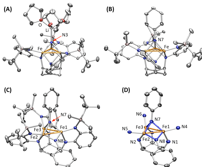
Figure 3.1. Solid-state structures for (A) [( tb L)Fe 3 (μ 3 -N)]Li(THF) 3 ( 3.2b ), (B) ( tb L)Fe 3 (μ 3 -NPh) ( 3.4 ), (C) ( tb L)Fe 3 (μ 3 -NPh)(μ 2 -NPh) ( 3.5 ) (core highlights of 3.5 in D) with the thermal ellipsoids set at the 50% probability level (hydrogen atoms and solvent molecules omitted for clarity; Fe orange, C gray, N blue, O red, Si pink, Li white). Selected bond lengths (Å) for ( 3.2b ): Fe–Fe, 2.4802(5); Fe–N3, 1.877(2); N3–Li, 1.990(6); for ( 3.4 ): Fe1–Fe2, 2.549(1); Fe1–Fe3, 2.502(1); Fe2–Fe3, 2.539(1); Fe1–N7, 1.935(5); Fe2–N7, 1.944(5); Fe3–N7, 1.944(5); for ( 3.5 ): Fe1–Fe2, 2.482(1); Fe1–Fe3, 2.966(1); Fe2–Fe3, 2.604(1); Fe1–N7, 1.973(4); Fe2–N7, 1.982(4); Fe3–N7, 1.904(4); Fe1–N8, 1.866(4); Fe2–N8, 1.848(4).
