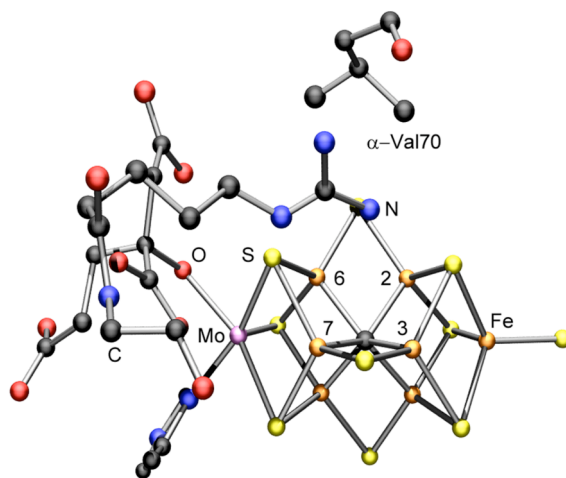
Figure 1.4. Nitrogenase FeMo-cofactor from Spatzal et al. 50 (Mo pink, Fe orange, C black, N blue, O red, S yellow) where the \alpha -Val70 residue and Fe(2367) tetrairon face are illustrated.
