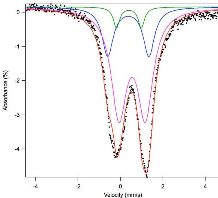
Figure 3.11. Crude zero-field Mössbauer spectrum of (^{ts}\text{L})\text{Fe}_3(\mu^3\text{-NH}) ( 3.3 ) obtained at 90 K prepared by method 2. Fitting parameters: \delta , |\Delta E_Q| ( \text{mm/s} ) component 1 (blue, 28%) 0.37, 1.94 ( \Gamma = 0.32 \text{ mm/s} ); component 2 (green, 12%) 0.40, 1.17 ( \Gamma = 0.18 \text{ mm/s} ); component 3 (pink, 60%) 0.55, 1.24 ( \Gamma = 0.45 \text{ mm/s} ). To obtain the fit, the parameters of components 1 and 2 representing 3.3 were fixed while component 3 was allowed to vary to obtain an approximate crude yield based on Fe content. Fitting the spectrum to a single quadrupole doublet yields the following parameters: \delta , |\Delta E_Q| ( \text{mm/s} ) 0.50, 1.4 ( \Gamma = 0.46 \text{ mm/s} ).
