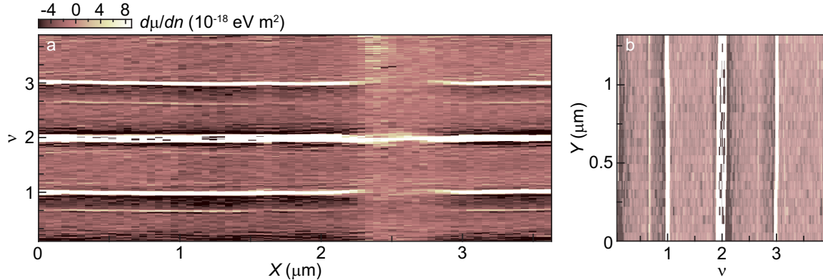
Figure 6.4: Inverse compressibility as a function of filling factor and position X (a) and Y (b). The sequence of FQH states does not vary with position.
