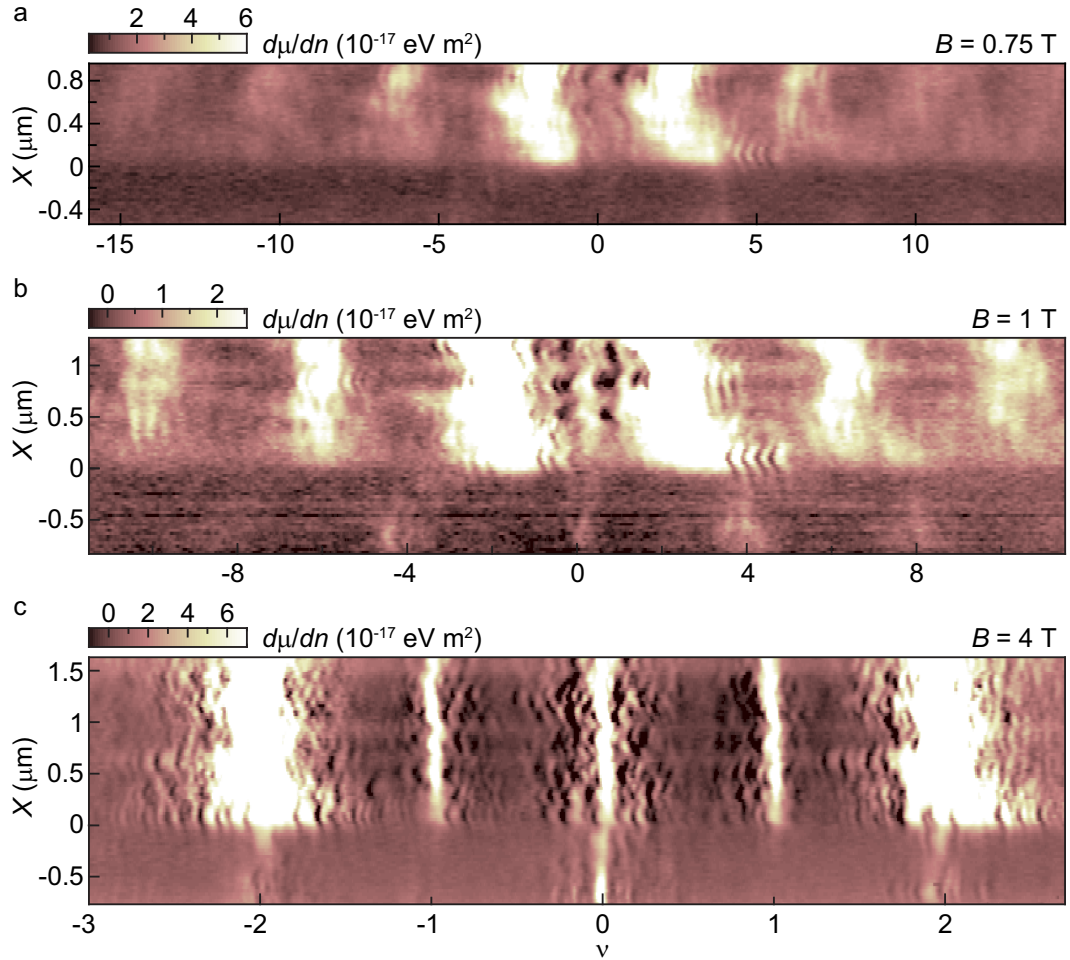
Figure 7.2: (a) Inverse compressibility d\mu/dn as a function of filling factor \nu and position X at B = 0.75 T (a), 1 T (b), and 4 T (c). Near the interface, the single-particle incompressible quantum Hall states weaken and broaden. The \nu = 0 state also weakens where the monolayer and bilayer meet, but the \nu = \pm 2 states get stronger and sharper on the bilayer side. In contrast to Fig. 7.1c, positive X corresponds to the monolayer side in this and subsequent experimental figures.
