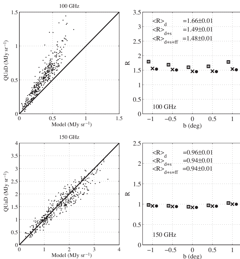
Figure 10. Left panels: QUaD pixel values plotted against signal-only simulations of the model including dust, synchrotron, and free–free as described in the text; top is 100 GHz, bottom is 150 GHz. Right panels: ratio of QUaD map pixel values to model predictions at 100 GHz (top) and 150 GHz (bottom), as a function of galactic latitude. Square symbols compare QUaD to the FDS dust model, crosses are dust+synchrotron, and dots correspond to dust+synchrotron+free–free.
